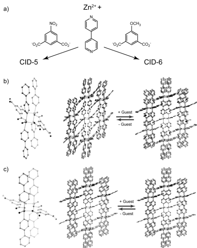
Figure 1. (a) Reaction schemes of CID-5 and CID-6. Crystal structures of the coordination environment around the \text{Zn}^{2+} ions and assembled 2D layer stacking of (b) CID-5 and (c) CID-6 before and after guest adsorption. Guests are omitted.
