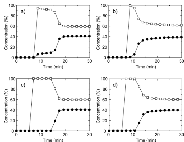
Figure 3. Breakthrough curves of \text{CH}_4/\text{CO}_2 mixture (60:40 (vol)) for (a) CID-5, (b) CID-6, (c) CID-5/6 ( x = 0.1 ) and (d) CID-5/6 ( x = 0.4 ). The open square is \text{CH}_4 and the closed circle is \text{CO}_2 . These were measured at 273 K, the total pressure was 0.80 MPa and the space velocity was 6 \text{ min}^{-1} .
