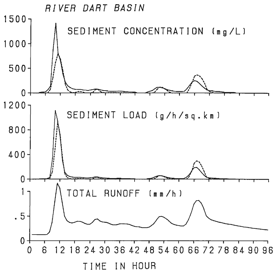
Fig. 7. Sediment concentration ( C_d ) and sediment load ( Q_{d1} ) as estimated by Eq. (13) (dashed lines) and as observed (continuous lines). The time starts at 12:00, 9 December, 1982.
