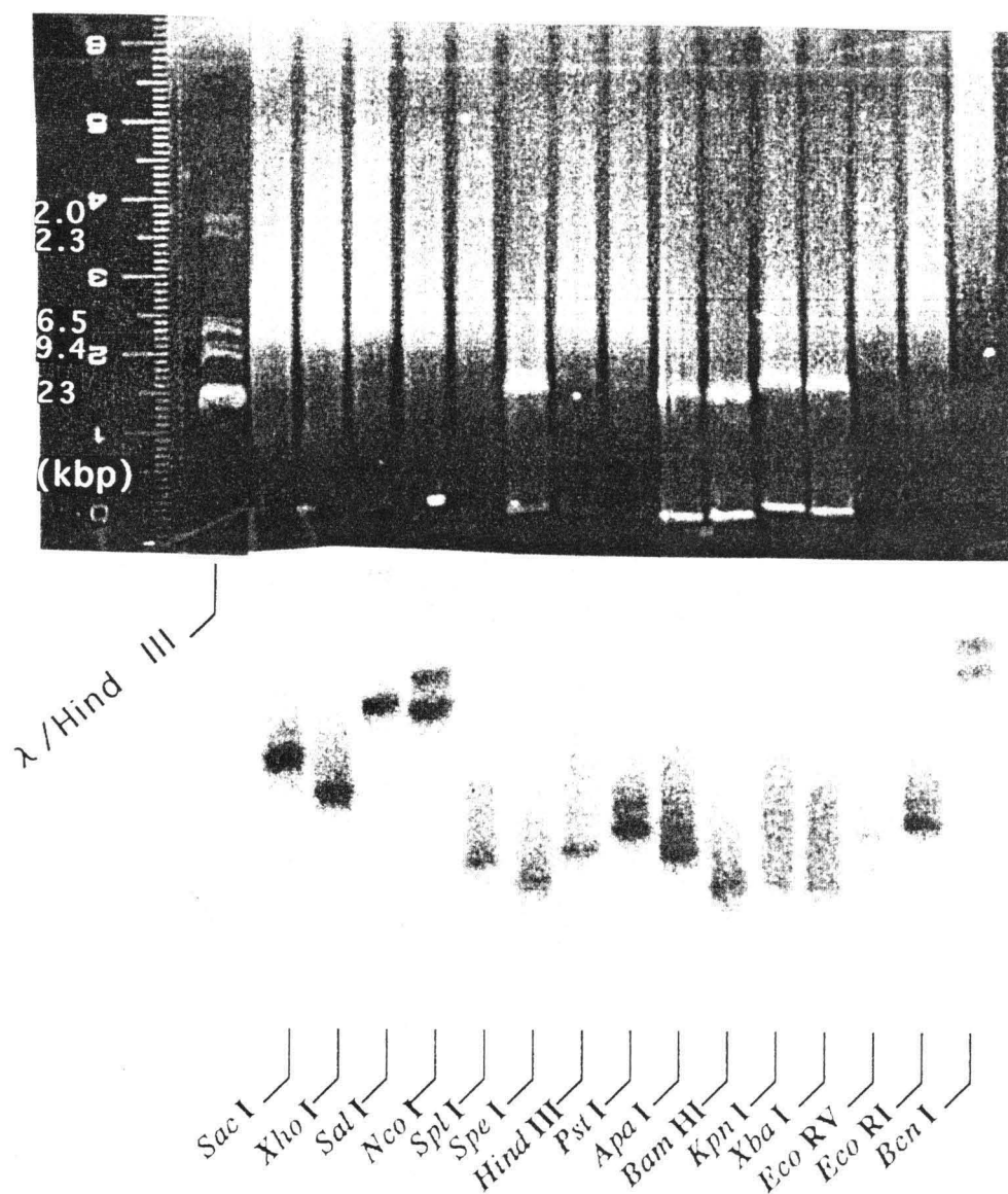
Figure 2 Southern hybridization for analysis of B.s. genomic DNA
