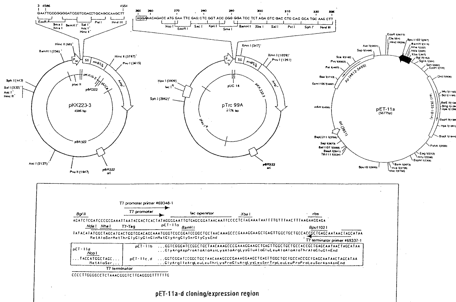
Figure 12 Strategy for overexpression of B.s. LysRS in E. coli
