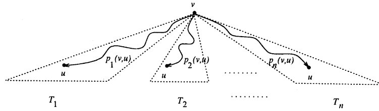
Figure 2: G is n -channel at node v if p_i(v, u) 's are node-disjoint for any u .
