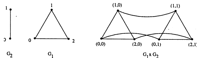
Figure 1: Example of a product network.
