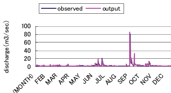
Fig.11 Discharge (Shorenji Dam, 2000)
