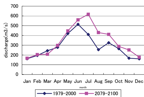
Fig.21 Monthly discharge (Hirakata)
