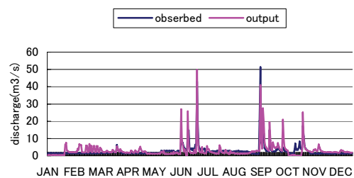
Fig.12 Discharge (Muro Dam, 2000)
