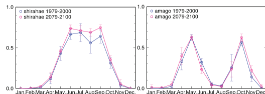
Fig.34 Adaptability (shirahae, amago)
