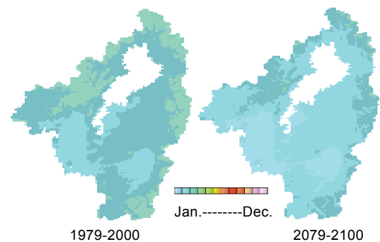
Fig.28 Pollen scattering season
