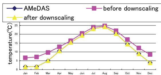
Fig.7 Monthly averaged temperature
