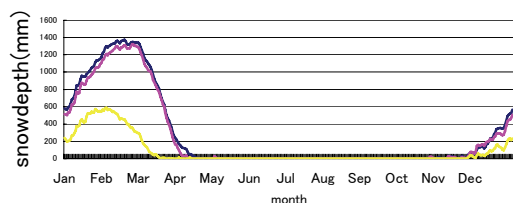
Fig.17 Snowdepth (Mt. Hakodate)
