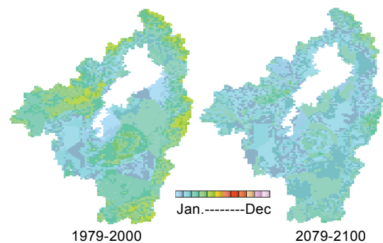
Fig.29 Pollen scattering season (Considering breaking of dormancy)
