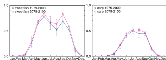
Fig.32 Adaptability (sweetfish, carp)
