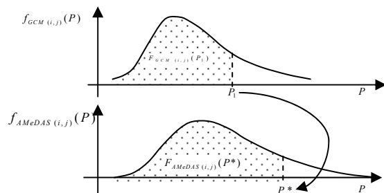
Fig.5 Pattern diagram of bias correction
