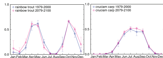
Fig.33 Adaptability (rainbow trout, crucian carp)
