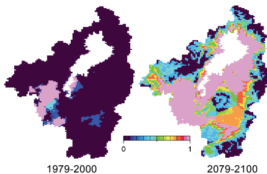
Fig.27 Adaptability of vegetation (subtropical)
