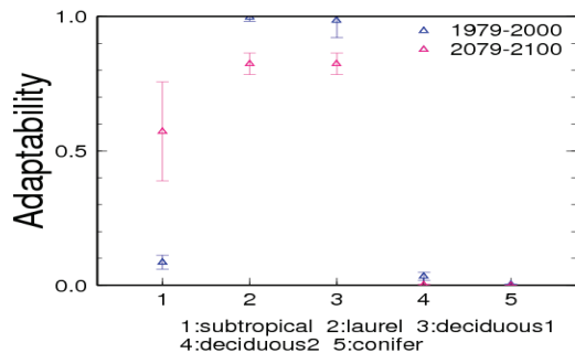
Fig.26 Adaptability of vegetation
