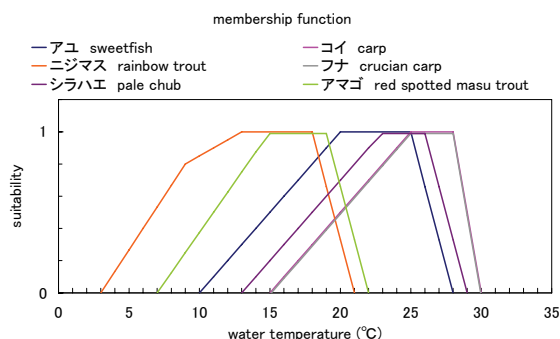
Fig.30 Membership function (water temperature)
