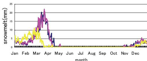
Fig.18 Snowmelt (Mt. Hakodate)
