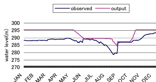
Fig.14 Water level (Muro Dam, 2000)
