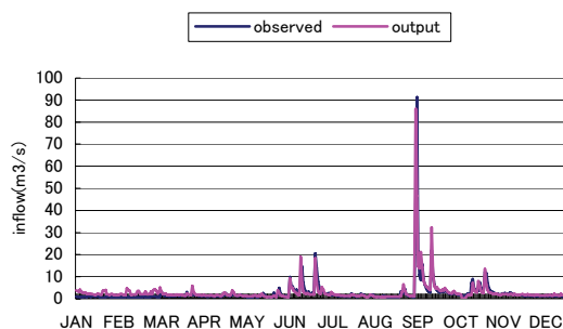
Fig.9 Inflow (Shorenji Dam, 2000)
