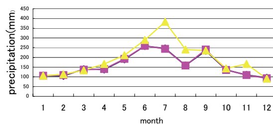
Fig.15 Monthly averaged precipitation
