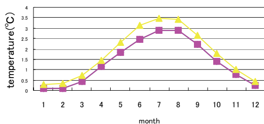
Fig.16 Monthly averaged temperature
