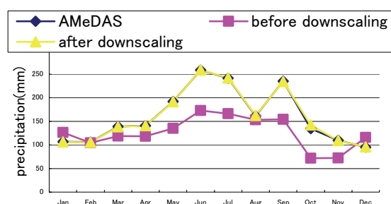
Fig.6 Monthly averaged precipitation
