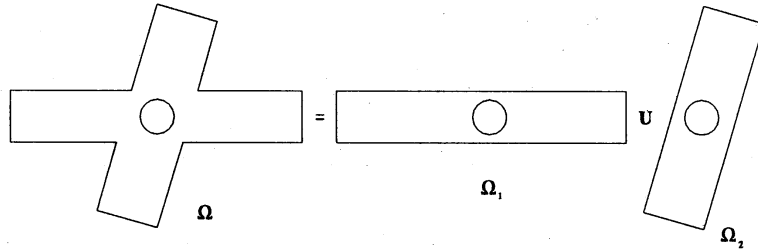
Figure 1: Overlapping domain decomposition
