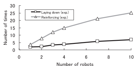
図10 ロボット数の増加と敷設・強化（コミュニケーション）回数の関係 Fig. 10 Relationship between the number of robots and the number of “laying down” and “reinforcing” times.
