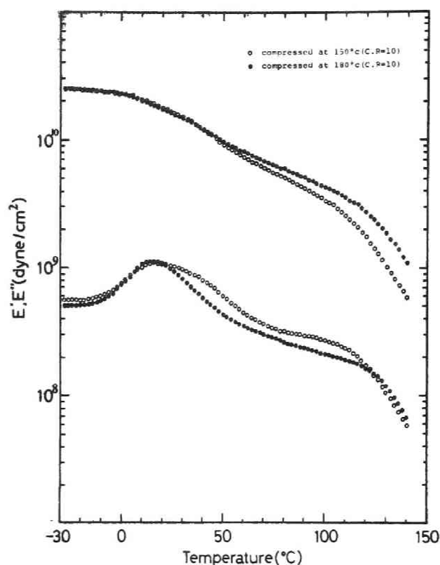
Fig.10. Temperature dependency of dynamic modulus E' and dynamic loss E'' for the crosslinked gel samples compressed at 150^{\circ}\text{C} and 180^{\circ}\text{C} .
