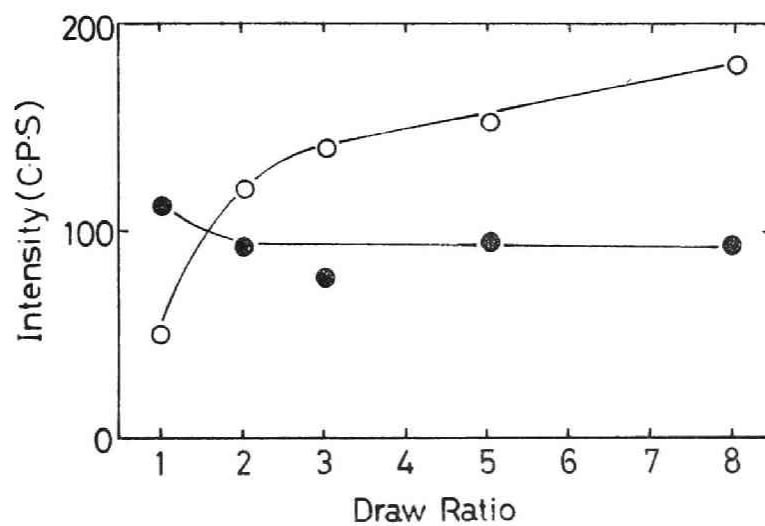
Fig. 7. Variation of the scattering intensity as a function of draw ratio for PVDF uniaxially stretched at 160°C (●) and at 180°C (○).
