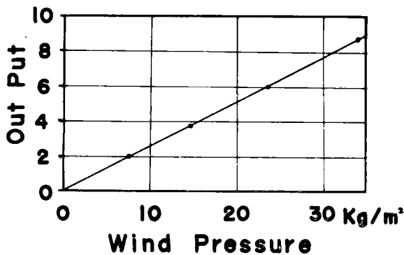
Fig. 9 Static characteristics of the pressure plate anemometer.
