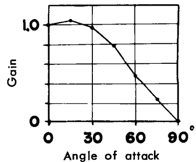
Fig. 10 Characteristics of the pressure plate anemometer to slant wind.
