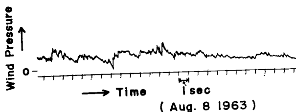
Fig. 16 An example of the trace of the pressure tube anemometer (AT-4)
