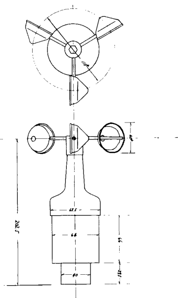
Fig. 21 Small anemometer AH-3.
