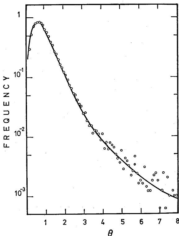
Fig. 1. Comparison of the distribution of random variates with the Molière theory.
