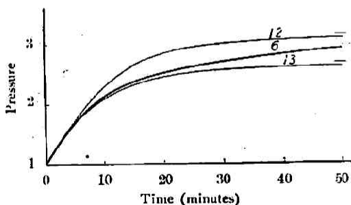
Fig. 7. 280°C { Exp. No. 6, ( \text{CH}_3\text{OH} )=76mmHg, ( \text{H}_2\text{O} )=0mmHg, Exp. No. 12, ( \text{CH}_3\text{OH} )=53mmHg, ( \text{H}_2\text{O} )=23mmHg, Exp. No. 13, ( \text{CH}_3\text{OH} )=56mmHg, ( \text{H}_2\text{O} )=21mmHg
