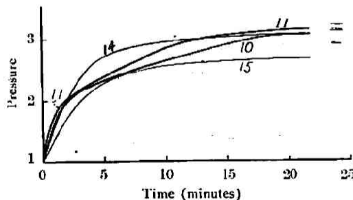
Fig. 8. 300°C { Exp. No. 10, ( \text{CH}_3\text{OH} )=61.4mmHg, ( \text{H}_2\text{O} )=0mmHg, Exp. No. 14, ( \text{CH}_3\text{OH} )=56.0mmHg, ( \text{H}_2\text{O} )=21mmHg, Exp. No. 11, ( \text{CH}_3\text{OH} )=39.0mmHg, ( \text{H}_2\text{O} )=0mmHg, Exp. No. 15, ( \text{CH}_3\text{OH} )=40.2mmHg, ( \text{H}_2\text{O} )=37.3mmHg
