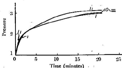
Fig. 6. 300°C { Exp. No. 1, ( \text{CH}_3\text{OH} )=70mmHg, Exp. No. 10, ( \text{CH}_3\text{OH} )=61mmHg, Exp. No. 11, ( \text{CH}_3\text{OH} )=39mmHg
