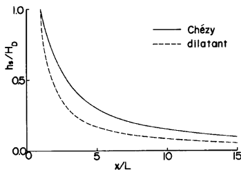
Fig. 14 Attenuation of depth at the shock front.
