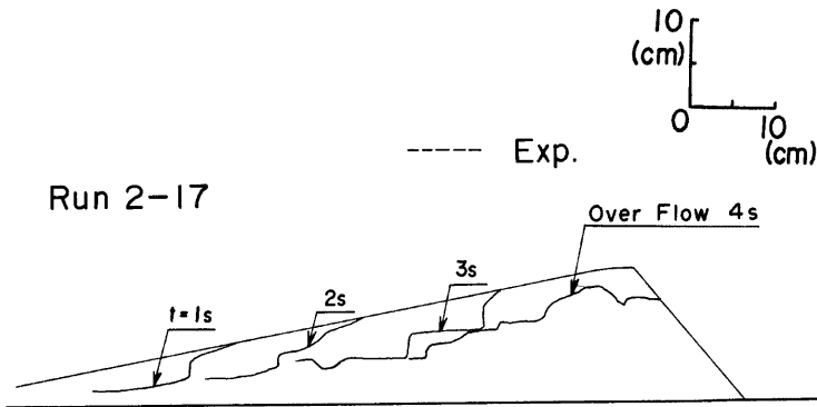
Fig. 6 Upstream advancement of failure in the dam-body.
