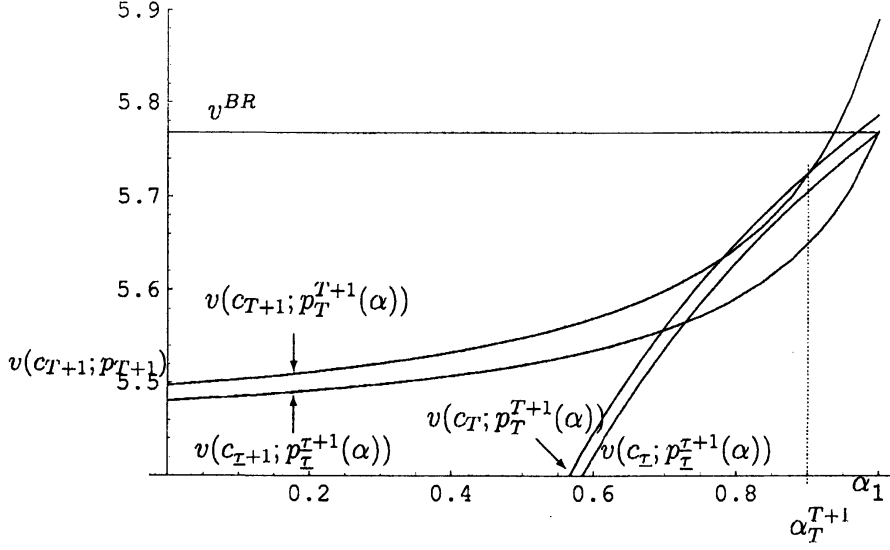
FIGURE 2. – The existence of a bimorphic NSD as T is slightly below \underline{\tau}(\delta) .
