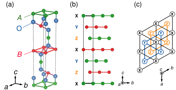
Figure 1: (a) Unit-cell crystal structure of delafossite ABO 2 . Both A and B ions form triangular lattices and stack along the c -axis in the sequence B-O-A-O-B. (b) Side view of the crystal structure. The oxygen ions above and below the A-site ions are not shown in this figure in order to focus on the layered structure of A and B atoms. The black lines indicate the unit cell. The symbols X, Y, and Z represent the stacking patterns of the layers. (c) Schematic drawing of the top view of the crystal structure. The definition of the symbols X, Y, and Z are the same as that in (b). These figures are generated by VESTA [17].
