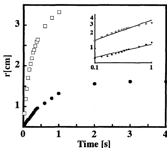
Fig.1: Time evolution of ethanol spreading on PAMPS solution (□) and gel (●). Concentrations are 0.2 wt.%. Inset figure is log - log representation.
