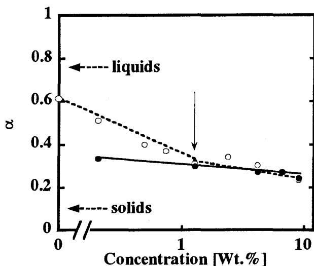
Fig.2: Ethanol spreading exponent \alpha as a function of concentration. Open and filled circles denote spreading on polymer solution and gels, respectively.
