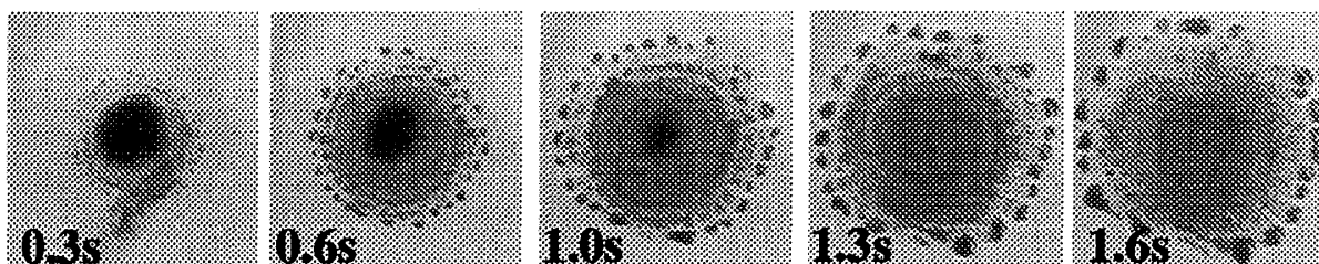
Fig.3 Snapshots of nonlinear pattern formation during spreading. Numbers in the figure indicate the spreading time.
