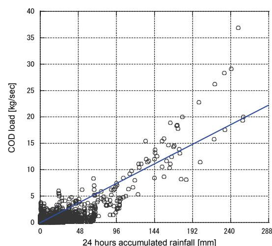
Fig.4 Scatter chart between an accumulate rainfall and COD load
