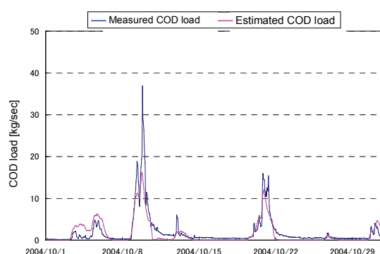
Fig.3 Estimated COD load
