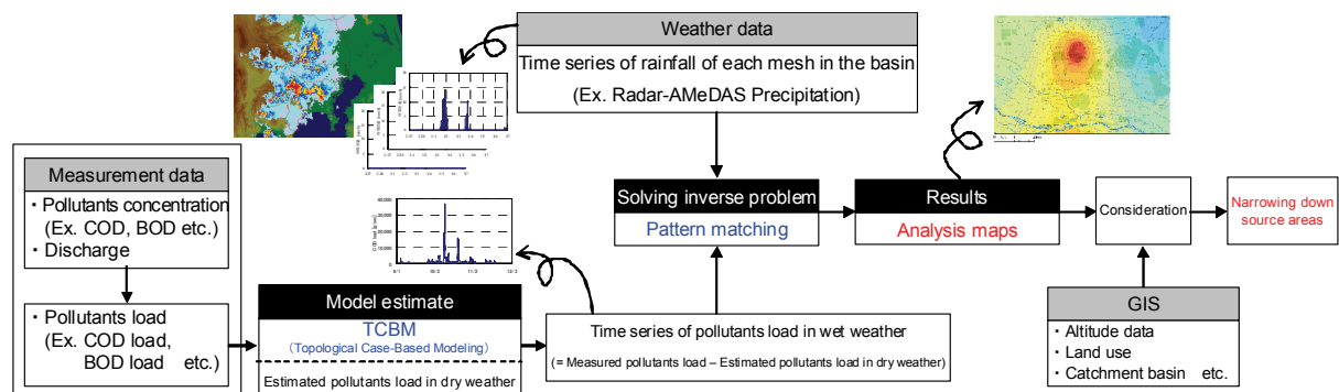
Fig.6 Overview of a method to specify source areas of environmental impacts
