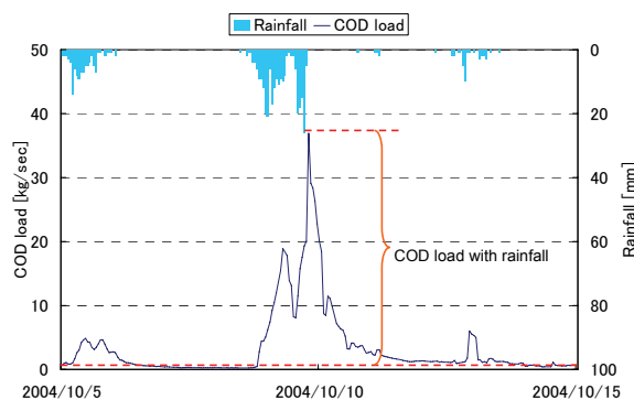
Fig.2 COD load with wet weather
