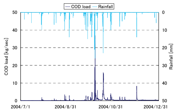
Fig.8 Measured COD load and Rainfall
