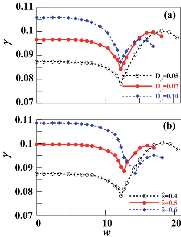
FIG. 6. The growth rate of resistive drift wave versus the magnetic island width w for different dissipation D_{\parallel} (a) or magnetic shear \hat{s} (b). The reference parameters are used except for \hat{s} = 0.4 (a), D_{\parallel} = 0.05 (b).
