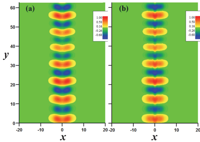
FIG. 2. Contour plots of potential (a) and density (b) perturbations of resistive drift wave in the simulation of Fig. 1. The corresponding parameters are D_{II} = 1.0 and \hat{s} = 1.0 .
