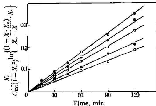
Fig. 2 Plots of \frac{X_e}{C_{KO}(1-X_e^2)} \ln \left\{ \frac{(1-X \cdot X_e)}{X_e - X} \cdot X_r \right\} vs. time at 0.68°C ○: 1 kg/cm², ●: 500 kg/cm², ▲: 1,000 kg/cm², ○●: 1,500 kg/cm², ●●: 2,000 kg/cm²
