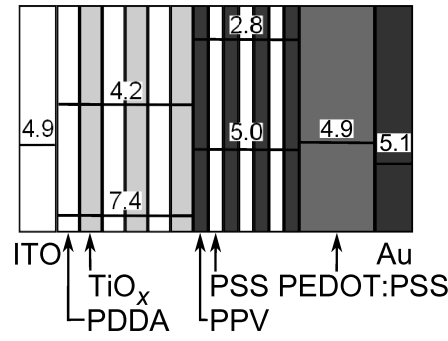
Figure 3–2. The layered structure and the energy diagram of the photovoltaic cell with the TiO x LbL film.
