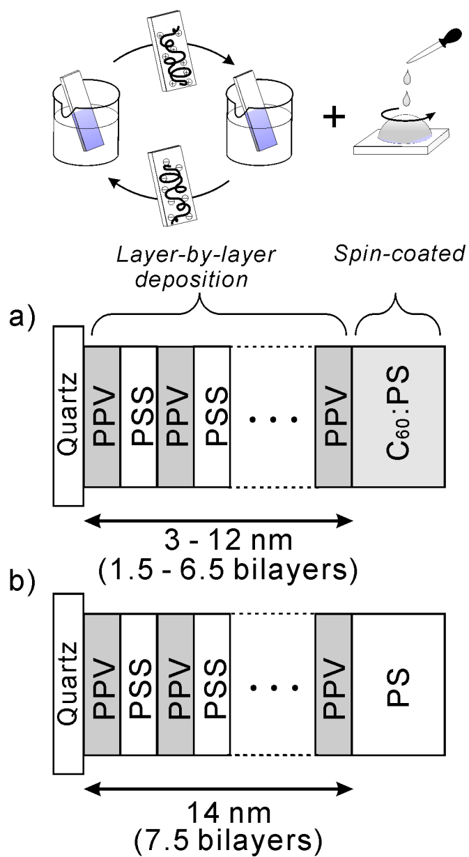
Figure 4–2. Schematic layered structures of the double-layered films employed for the quenching measurements. a) (\text{PPV/PSS})_n/\text{PPV}|\text{C}_{60}\text{:PS} , b) (\text{PPV/PSS})_n/\text{PPV}|\text{PS} . The monolayer thickness in (\text{PPV/PSS})_n/\text{PPV} was 0.9 nm for PPV and 1.0 nm for PSS.
