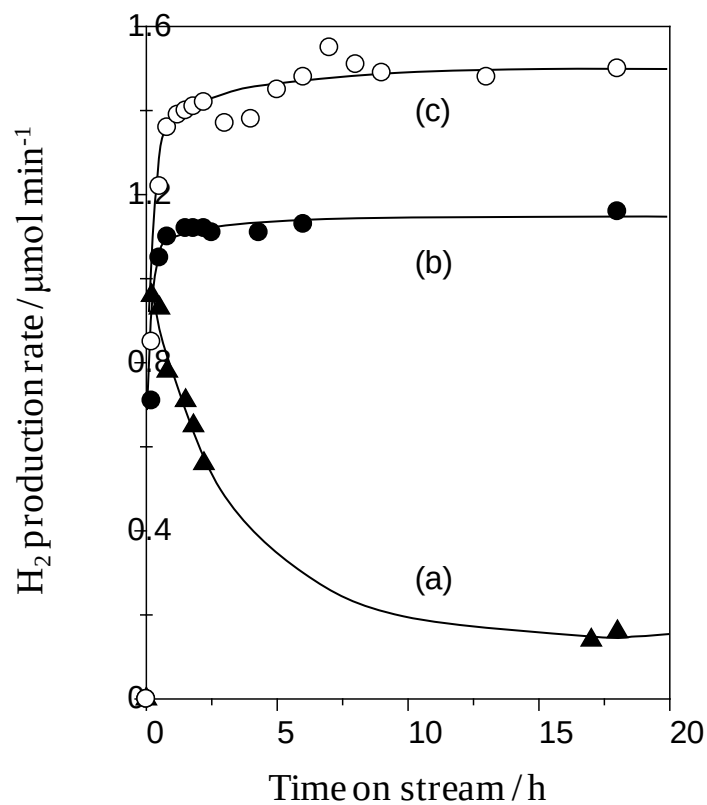
Fig. 7 Time course of the \text{H}_2 production rate on the \text{Pt}/\text{NaTaO}_3\text{:La} samples, on which Pt was loaded (a) by photodeposition method, (b) by photodeposition method followed by calcination and reduction at 773 K, and (c) by impregnation method followed by calcination and \text{H}_2 reduction at 773 K. Data were from [32].
