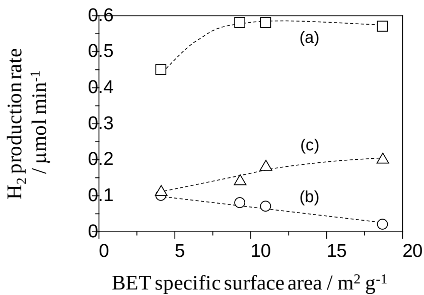
Fig. 6 Effect of the BET specific surface area of the \beta\text{-Ga}_2\text{O}_3 samples on the hydrogen production rate (a) in the flow of both water vapor and methane (the PSRM), (b) in the flow of water vapor (the WD) and (c) in the flow of methane (the MD). Data were from [35].
