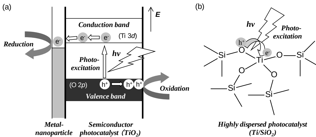
Fig. 1 Photoexcitation of (a) semiconductor photocatalyst (TiO 2 ) and (b) highly dispersed photocatalyst (Ti/SiO 2 ).
