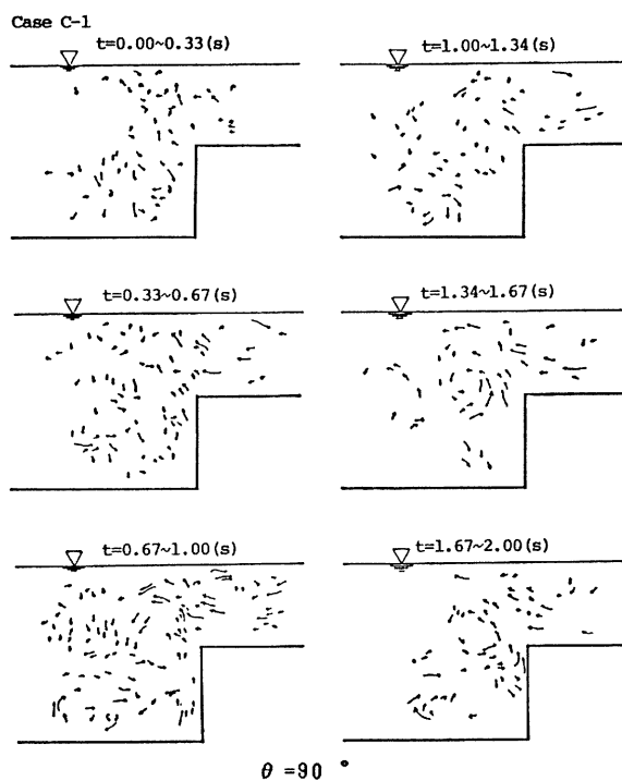
Fig. 2 Pass lines of neutral tracers in a cross section ( \theta=90^\circ )
