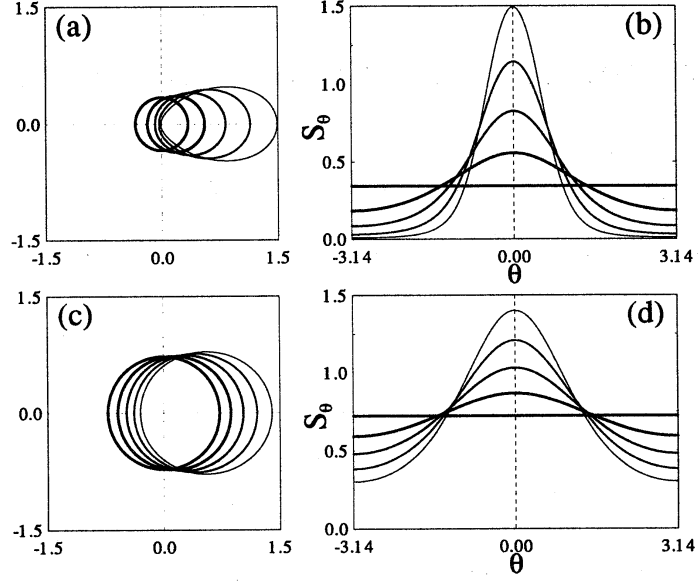
FIG. 2. Entropic density for coherent states [figs. (a) and (b)] and for superpositions of coherent signal and noise with \langle n_{\text{ch}} \rangle = 10 [figs. (c) and (d)] for the coherent amplitude \alpha_0 equal to: 0 (thickest solid line), 0.4, 0.8, 1.2, 1.6 (thinnest line).
