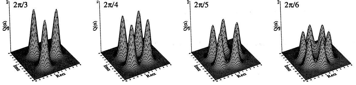
FIG. 6. Husimi Q -function for Schrödinger cat-like states generated in Kerr medium at different evolution times \kappa t = 2\pi/N for the field initially coherent with the mean photon number |\alpha_0|^2 = 9 .
