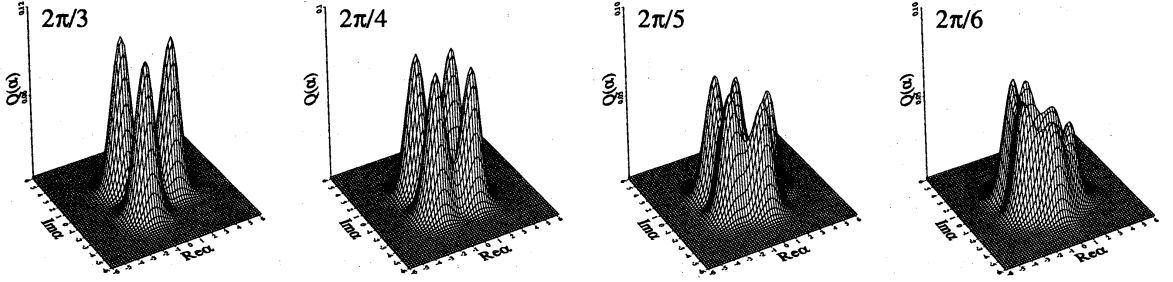
FIG. 7. Same as in Fig. 6, but for the initial condition |\alpha_0|^2 = 4 .
