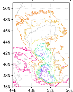
BATHYMETRY (GEBCO) Caspian Sea
