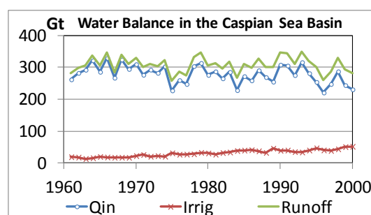
Fig.7 Water balance in the Caspian Sea Basin
