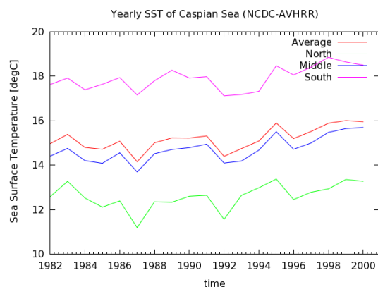
Fig.11 Historical change of annual averaged sea surface temperature
