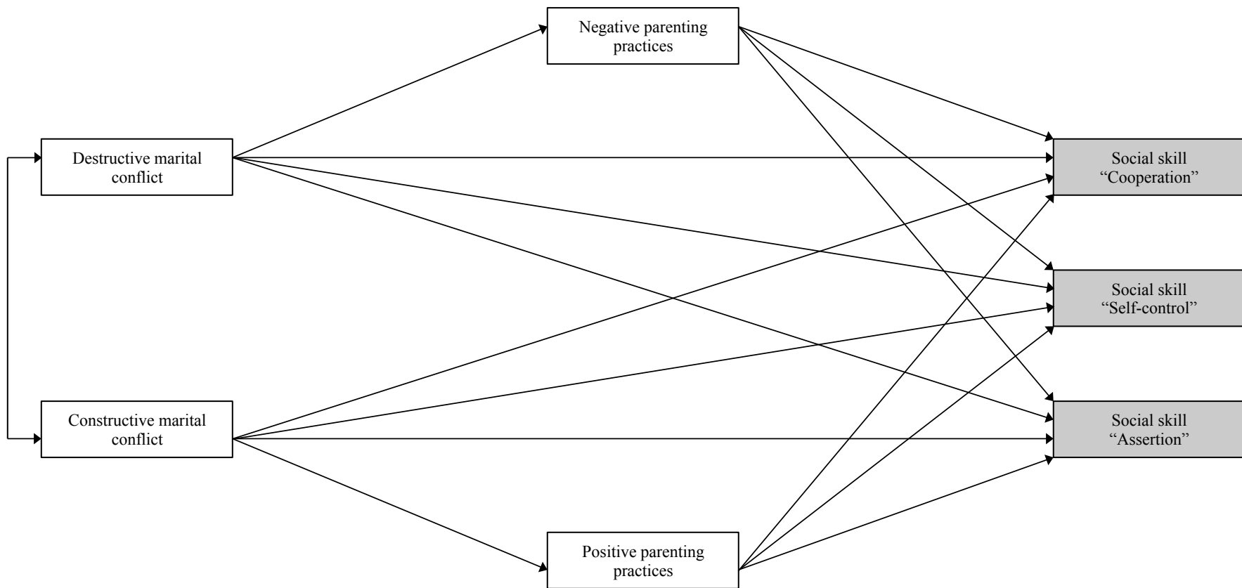
Figure 1. Hypothesized Model
