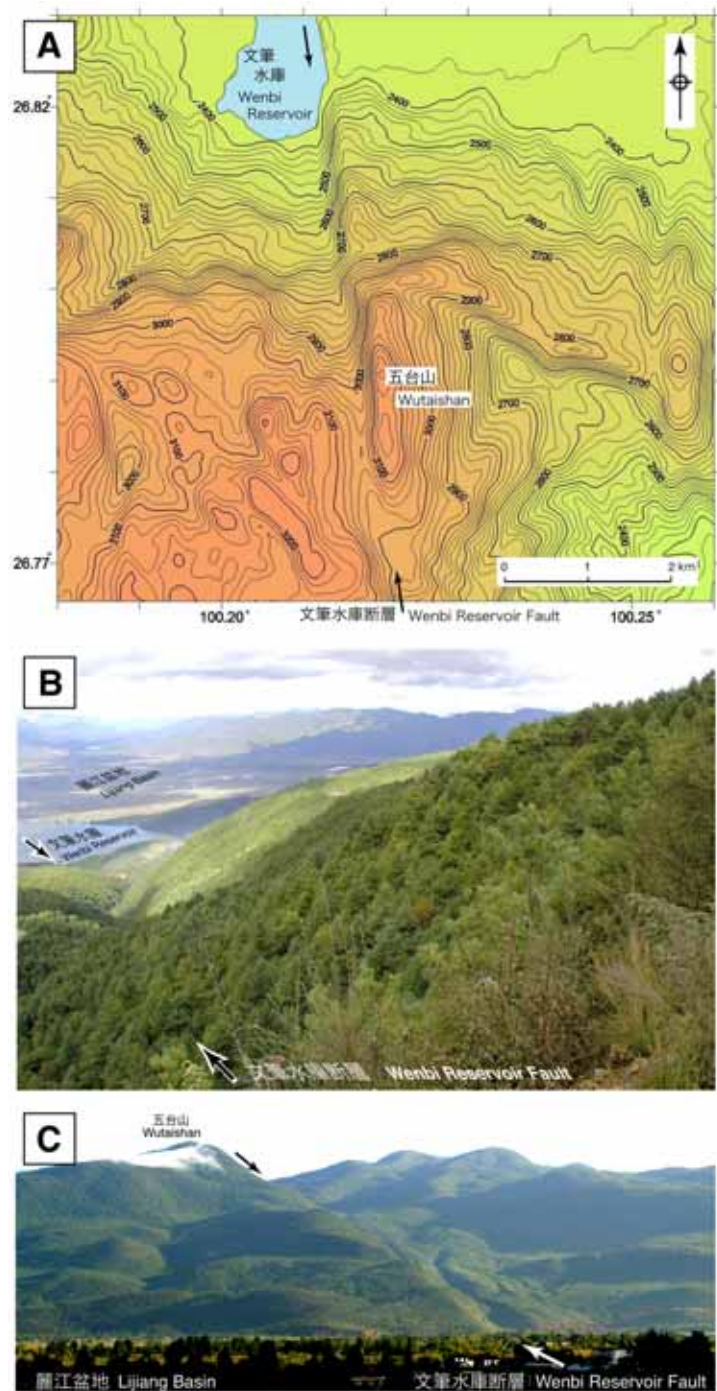
Fig. 9 Wenbi Reservoir Fault. A: Geomorphic structure of the marginal slope of the southwestern Lijiang Basin. Imaging the SRTM 3" mesh data of NASA < http://www2.jpl.nasa.gov/srtm/ >. B: Scarp surface of the Wenbi Fault (a northward view from a pass west of Wutaishan). C: Fault-scarp of the Wenbi Fault (a southward view from the Lijiang Basin).
