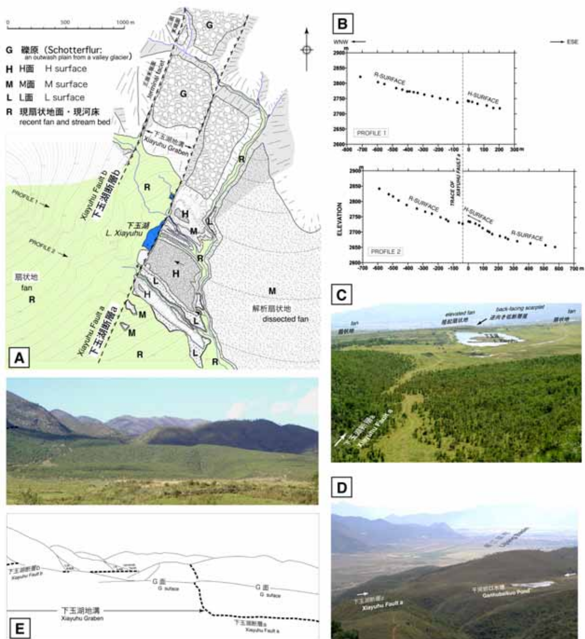
Fig. 7 Xiayuhu Faults. A: Geomorphologic structure around the Lake Xiayuhu at the northwestern corner of the Lijiang Basin. See Fig. 6 for location. B: Geomorphic profiles traversing the Xiayuhu Fault a, through differential GPS with AshtechProMark2. See Fig. 7A for location. C: Back-facing scarplet and fan displacement along the trace of the Xiayuhu Fault a, a view from the north. D: Back-facing scarplet along the northern trace of the Xiayuhu Fault a at the Ganhubaikuao Pond. See Fig. 6 for the location of the pond. E: Xiayuhu Graben, a northward view from the northern end of the Lijiang Basin.
