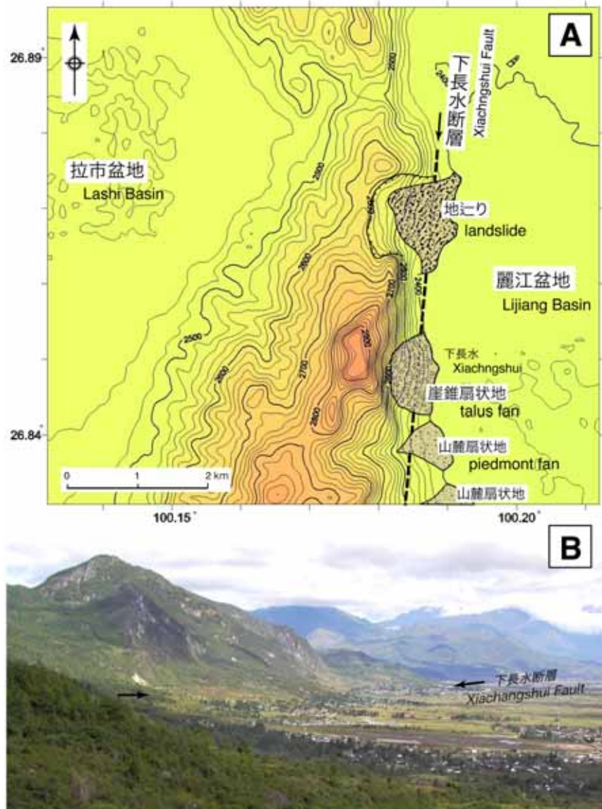
Fig. 8 Xiachangshui Fault. A: Geomorphic structure of the west margin of the southern Lijiang Basin. Imaging the SRTM 3" mesh data of NASA < http://www2.jpl.nasa.gov/srtm/ >. B: Fault-scarp of the Xiachangshui Fault (a northwesterly view from the southern margin of the Lijiang Basin).
