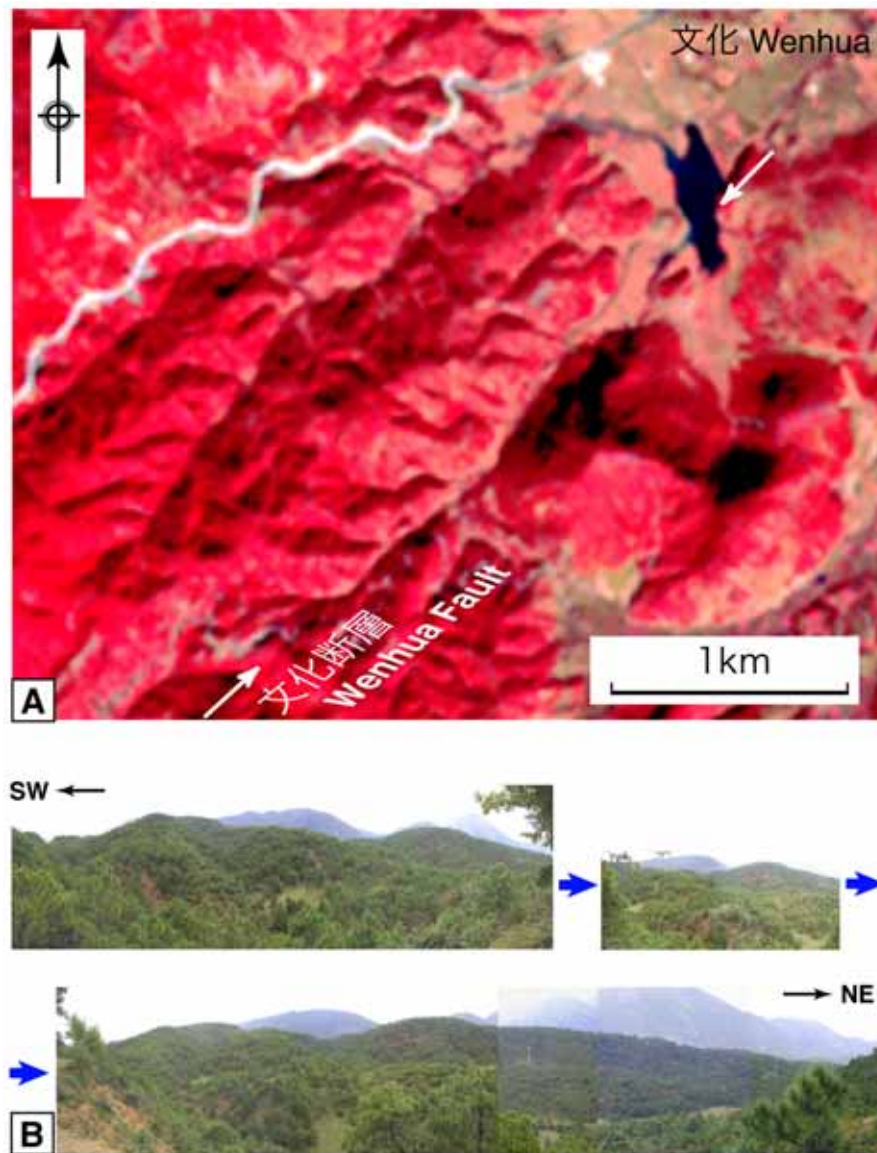
Fig. 12 Wenhua Fault. A: ASTER image showing the left-lateral displacement of the Wenhua Fault to the southwest of Wenhua. From ortho data Level-3A01 produced by ASTER GDS < http://www.science.aster.ersdac.or.jp/index.html >. B: Systematic left-lateral bend of spurs and streams on the northwest wall of the Wenhua Fault.
