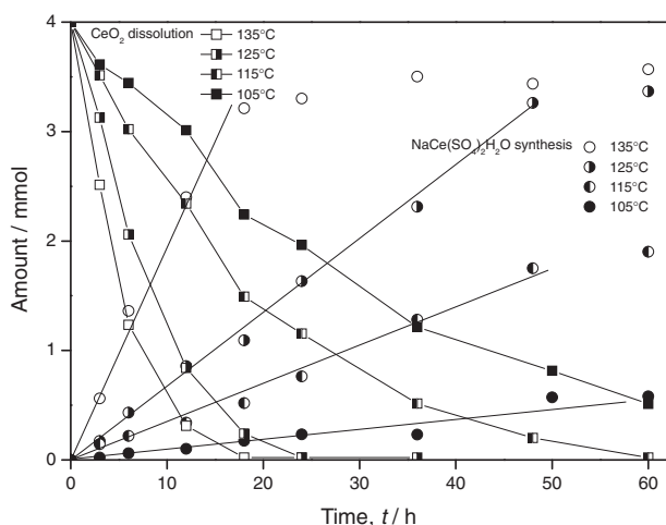
Fig. 4 Effect of reaction temperature on cerium oxide dissolution and sodium cerium sulfate synthesis kinetics in 1.0 mol/dm 3 sodium sulfate and 10 mol/dm 3 sulfuric acid solutions at 105–135°C.
