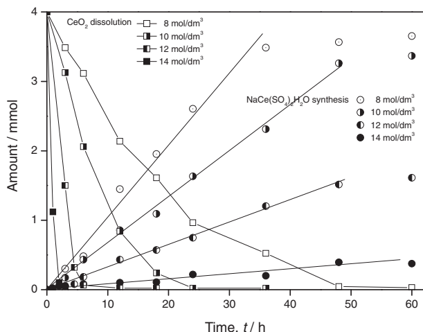
Fig. 3 Effect of sulfuric acid concentration on cerium oxide dissolution and sodium cerium sulfate synthesis kinetics in 1.0 mol/dm 3 sodium sulfate and 8–14 mol/dm 3 sulfuric acid solutions at 125°C.
