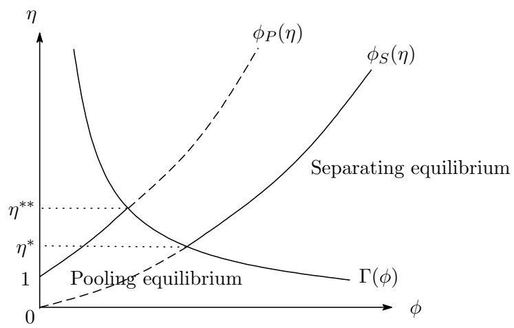
Figure 2: Nash Equilibria
