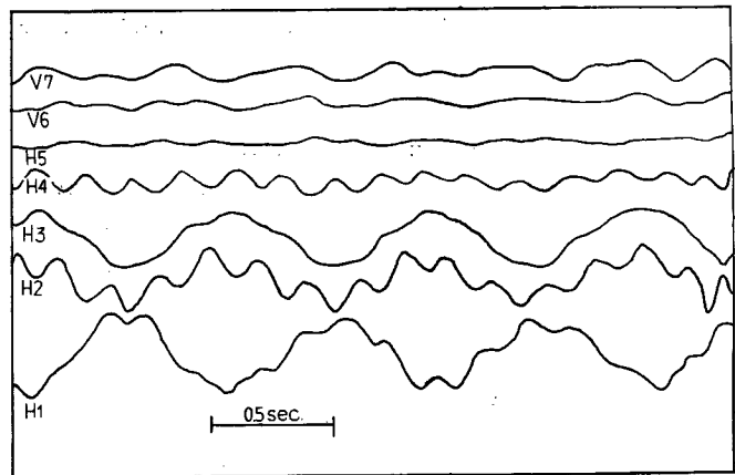
Fig. 2 (A) A record of the horizontal and vertical vibrations of the stack under the natural wind ; the two curves above in the figure show the vertical vibrations at the base of stack, and other five curves show the horizontal vibrations of stack
