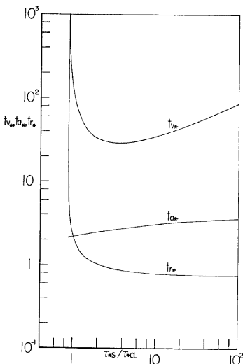
Fig. 12 Dimensionless relation of migrating, accelerating and departing time ( t_{e*} , t_{a*} and t_{r*} respectively) to the ratio of shear stress to critical one ( \tau_{*s}/\tau_{*cL} ).
