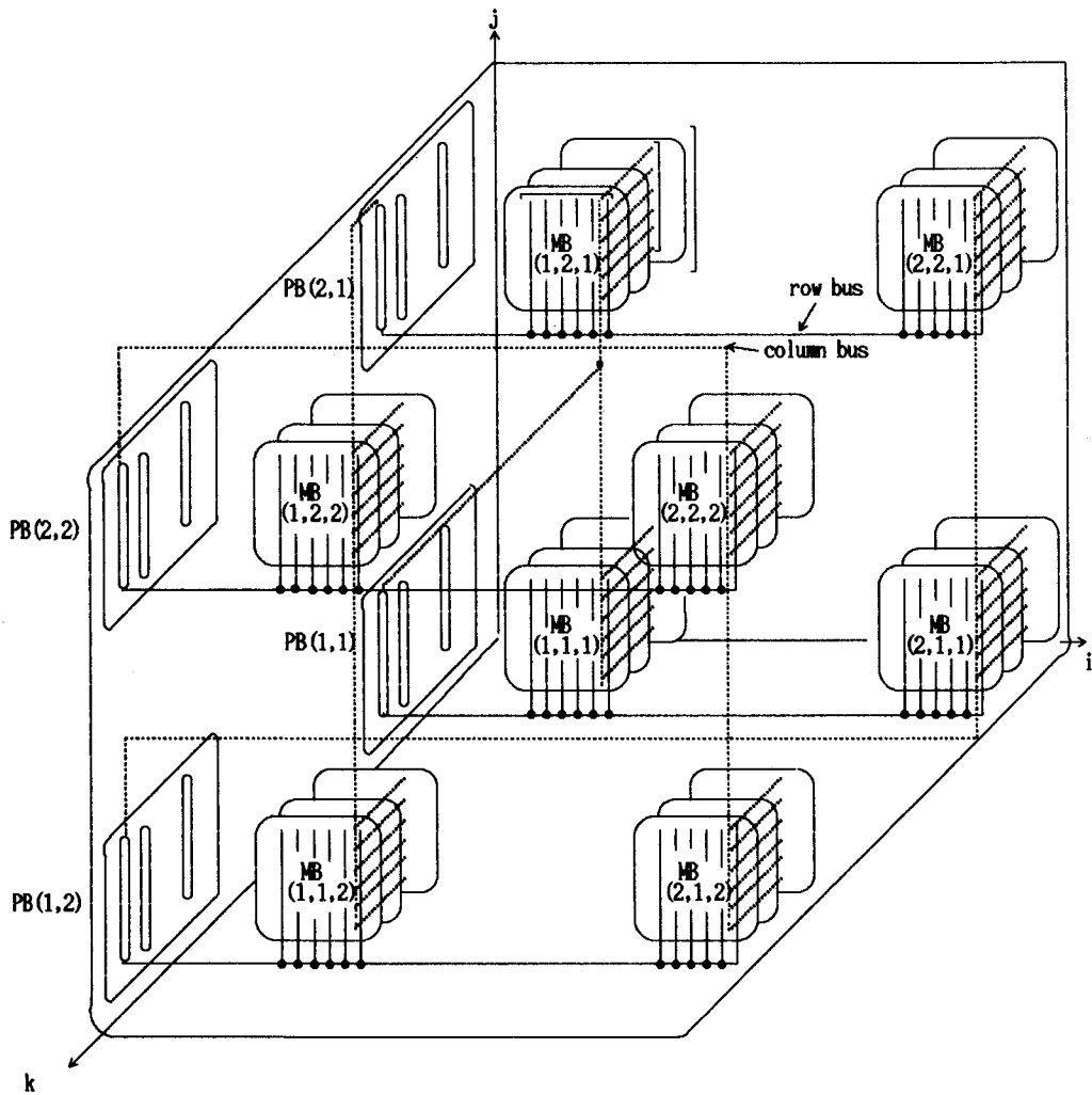
Fig. 5 ( 2^2, 2^3 ) extended system.
