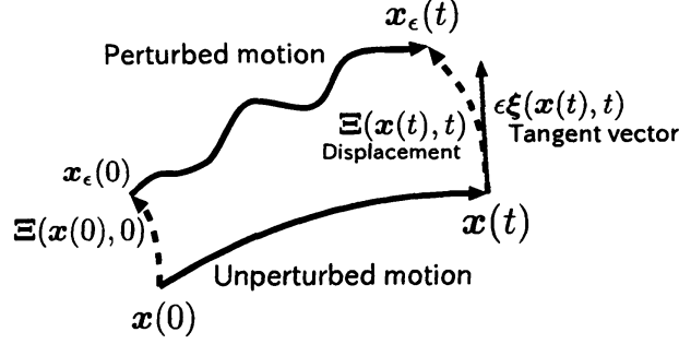
FIG. 2: Unperturbed and perturbed orbits of a fluid element
