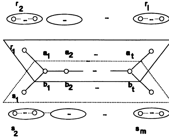
Figure 7: Confluence of the two relations \rho_1 and \sigma_1
