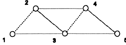
Figure 1: Zadori's semirigid system z_k of three equivalence relations ( n = 5, k = 2 )
