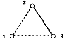
Figure 5: z_1 : the semirigid triangle
