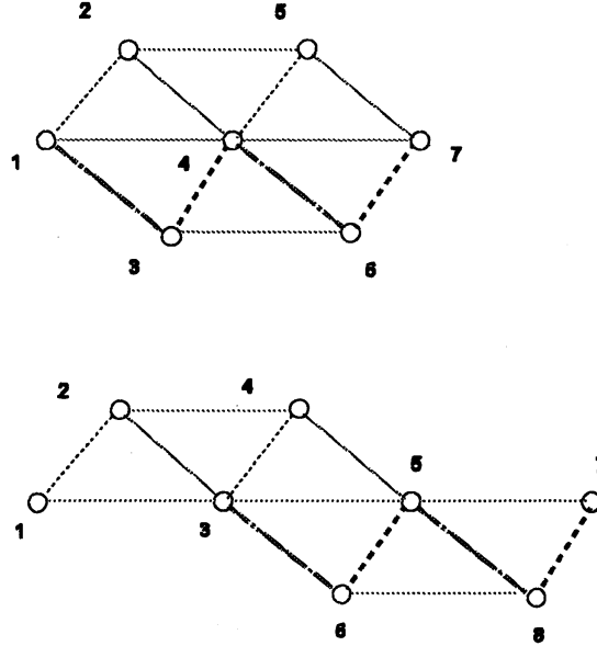
Figure 8: Two semirigid systems obtained by the composition (with 5 partitions).
