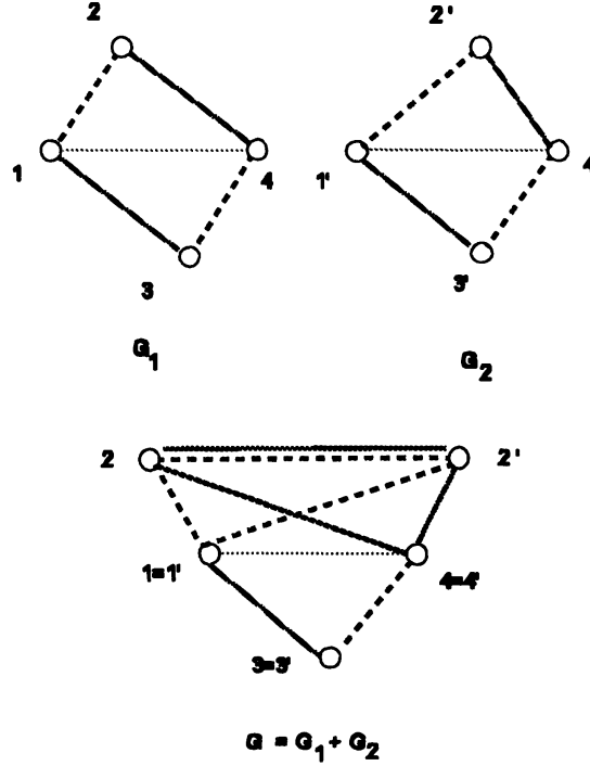
Figure 11: Non-orthogonality may occur by gluing.
