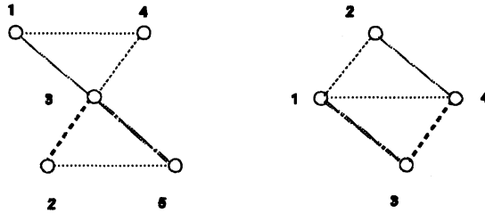
Figure 5: z_1 : the semirigid triangle
