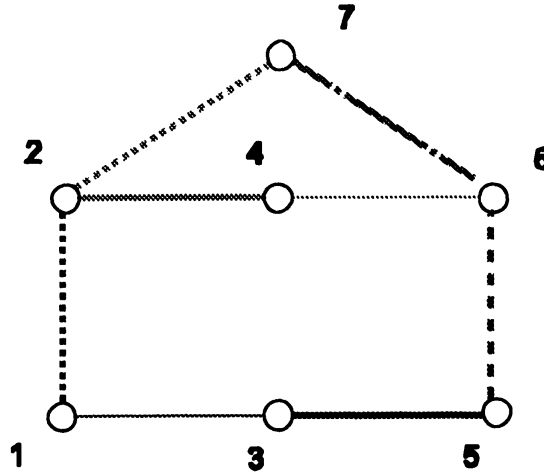
Figure 9: Gluing subsets with distinctively-colored edges yields a semirigid graph.
