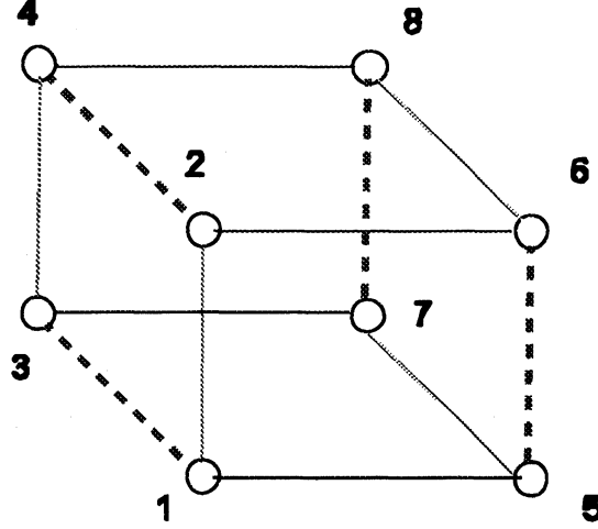
Figure 2: There is no second path between nodes 2 and 6.
