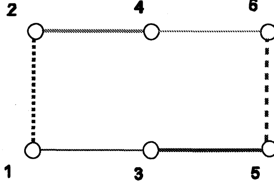
Figure 4: N -loop with distinctly colored n -edges is semirigid.
