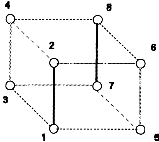
Figure 3: Non semirigid doubly connected graph (6 colors)
