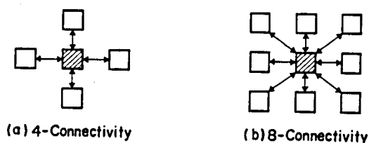
Figure 3-22 4- and 8-Connectivity
