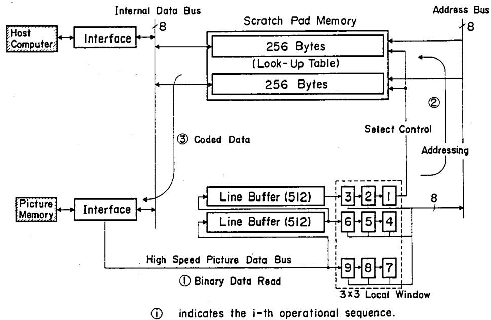
Figure 3-21 Logical Filtering Module
