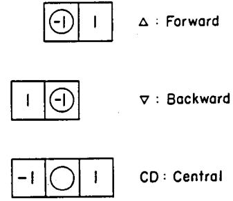
Figure 2-17 First-Order Forward, Backward and Central Difference Operators
