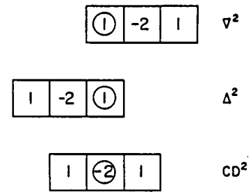
Figure 2-18 Second-Order Difference Operators
