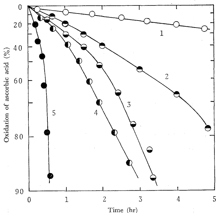
Fig. 1. Autoxidation of ascorbic acid 1: non-buffered, 2: pH=7.0, 3: pH=8.0, 4: pH=9.0, 5: pH=10.0 ascorbic acid: 5 \times 10^{-5}M , temp.: 21 \sim 23^{\circ}C
