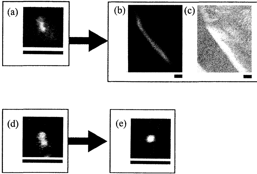
Figure 1: DNA conformations induced by the existence of PEG. All scale bar represents 5 \mu m . (a) coiled DNA molecule in concentrated DNA solution (DNA 20 \mu g/ml , PEG 170 mg/ml , NaCl 100 mM ). (b) elongated state of DNA molecule embedded in a liquid crystal, which was generated by a phase segregation to DNA rich phase and PEG rich phase from uniform phase.(DNA 20 \mu g/ml , PEG 230 mg/ml , NaCl 100 mM ). (c) the polarization microscopic image of the identical region as (b). (d) coiled DNA molecules in dilute DNA solution (DNA 0.1 \mu g/ml , PEG 170 mg/ml , NaCl 100 mM ). (e) compact state of DNA in dilute DNA solution(DNA 0.1 \mu g/ml , PEG 230 mg/ml , NaCl 100 mM ).
