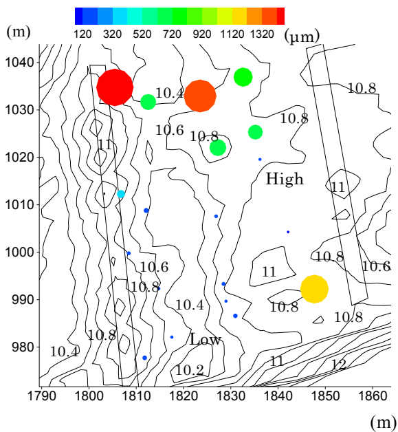
Fig.11 Mean grain size distribution in the groin bay of the Kizu site
