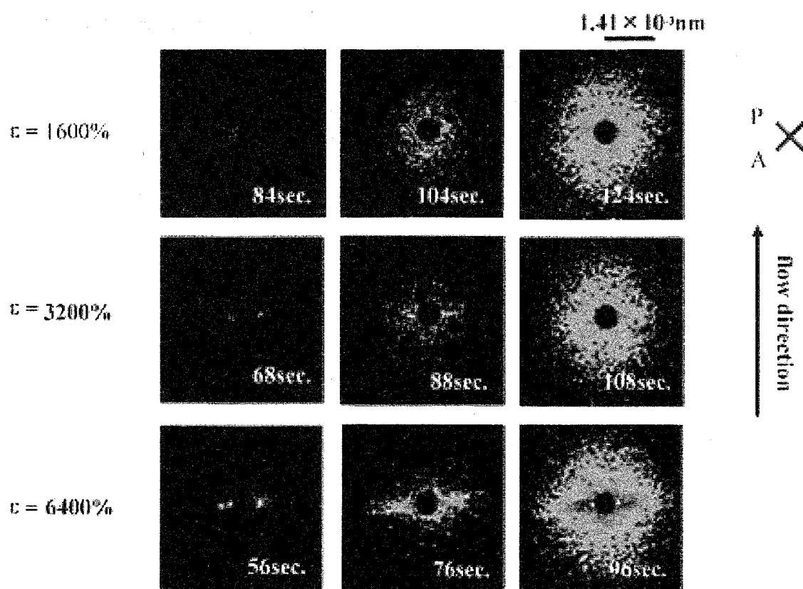
Fig. 5. Time evolution of 2D DPLS pattern form PE during the crystallization process at 129 °C after pulse shear.
