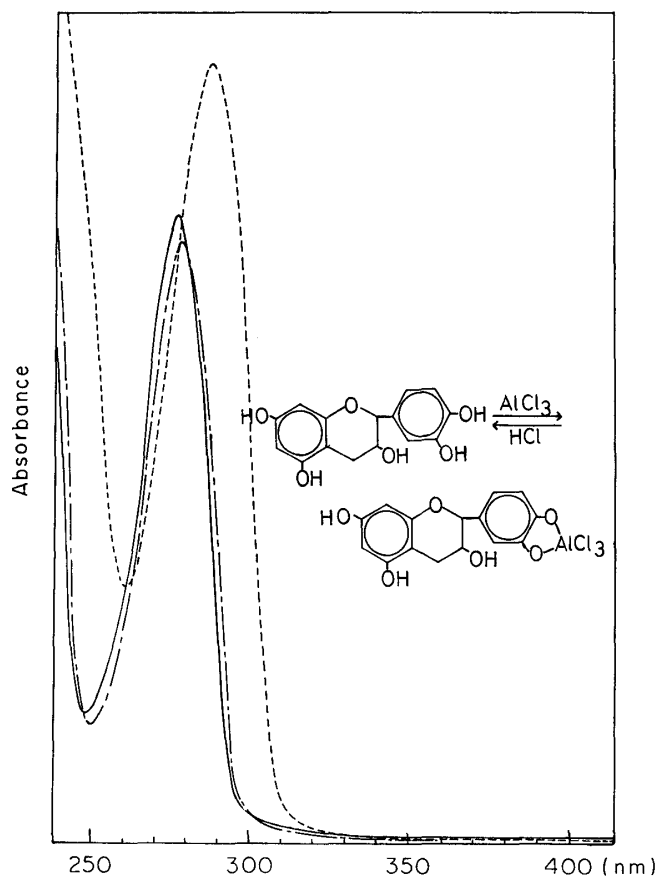
Fig. 5. Effect of \text{AlCl}_3 on the spectrum of d -catechin.
