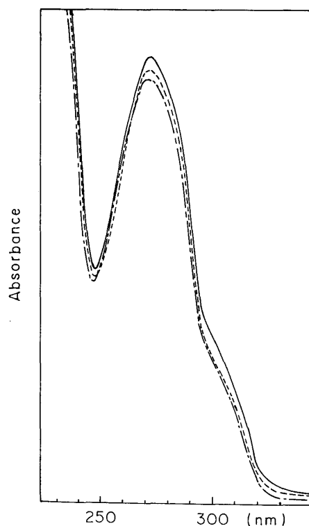
Fig. 6. Effect of \text{AlCl}_3 on the spectrum of coniferyl alcohol DHP.
