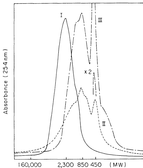
Fig. 3. Molecular weight distribution of I — Precipitate, II ---- \text{Et}_2\text{O} soluble and III — EtOAc soluble fractions in dehydrogenative polymerization of coniferyl alcohol and d -catechin.
