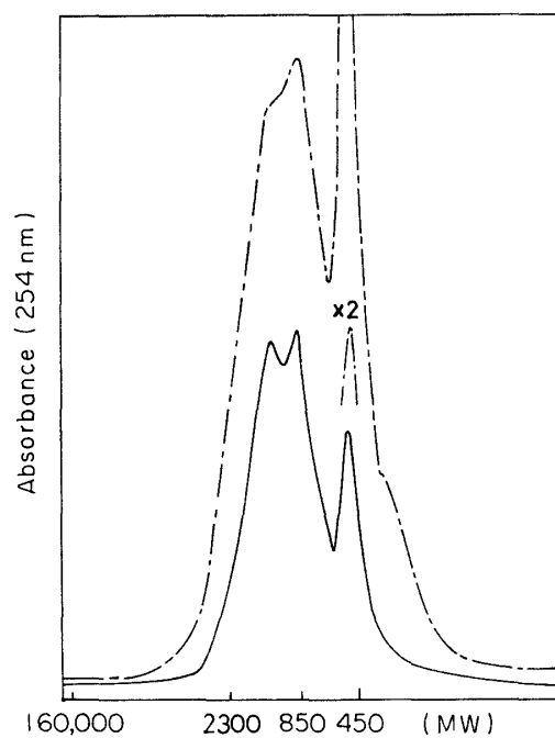
Fig. 4. Molecular weight distribution of EtOAc soluble fractions of the reaction mixture during dehydrogenation. ..... after 12 hrs ---- after 30 hrs
