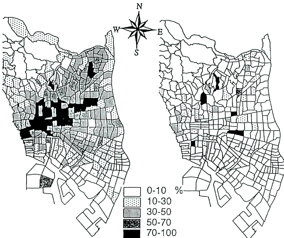
Fig. 13 Distribution of collapse ratio of wooden houses in Nishinomiya
