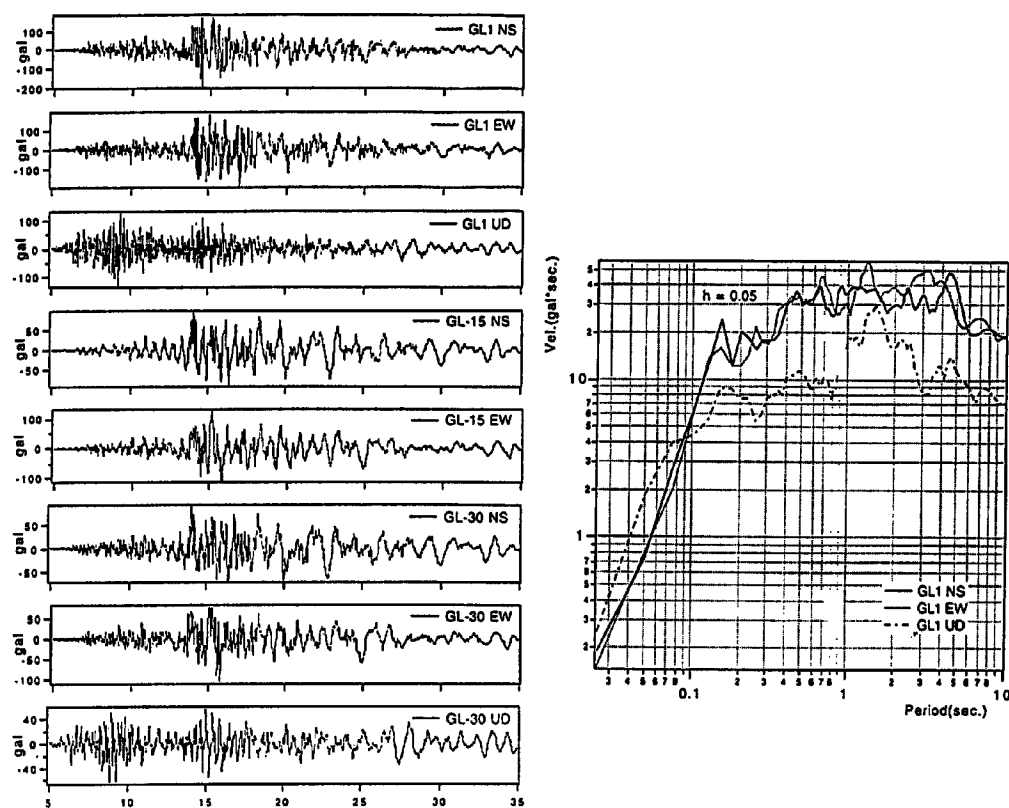
Fig. 2 Acceleration records at the surface ground and basement of the filtration building in Hirakata, Osaka and response spectrum with 5 % damping of the record at surface ground
