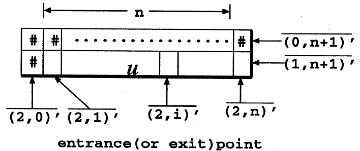
Figure 5: An Illustration for u(\#) .
