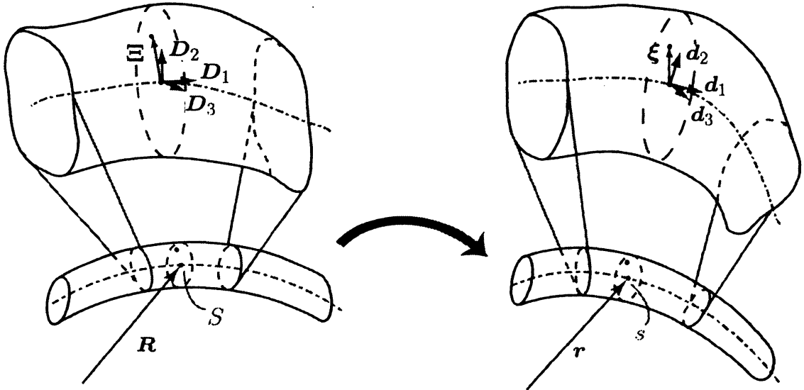
Figure 2: Illustration of the reference and current configurations of the Cosserat rod.
