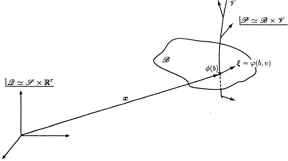
Figure 1: Illustration of the continuum with microstructure, \mathcal{P} \simeq \mathcal{B} \times \mathcal{V} , embedded into the ambient bundle, \mathcal{Q} \simeq \mathcal{S} \times \mathbb{R}^r , and its local coordinates in \mathcal{Q} .
