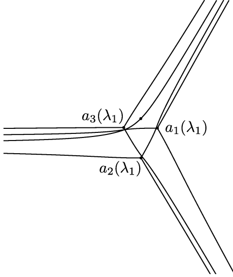
Figure 16. The ordinary Stokes curves and one particular new Stokes curve of the \text{AKT}_{\lambda_1} equation; here and in what follows the dot on a new Stokes curve designates the virtual turning point from which it emanates.
