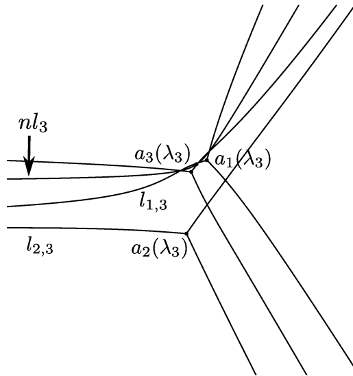
Figure 20. The Stokes geometry in question of the \text{AKT}_{\lambda_3} equation.
