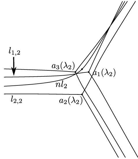
Figure 19. The Stokes geometry in question of the \text{AKT}_{\lambda_2} equation.
