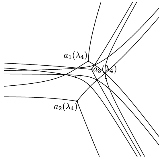
Figure 30. The Stokes geometry in question of the \text{AKT}_{\lambda_4} equation.
