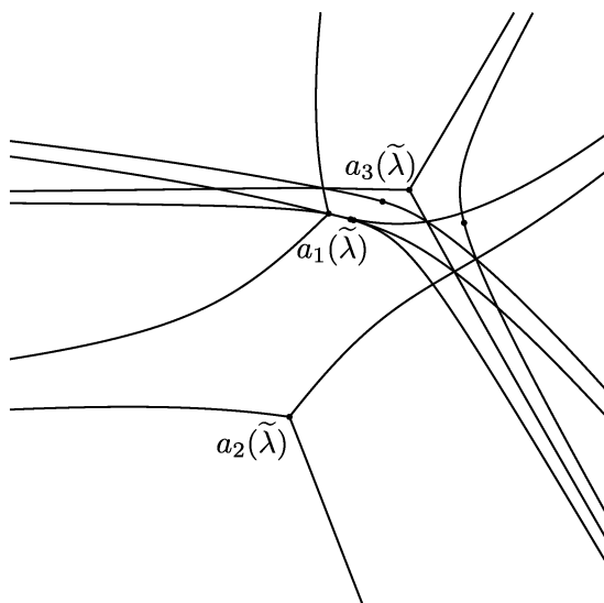
Figure 34. New type of degeneracy for the Stokes geometry of the \text{AKT}_{c_2} equation. (An enlarged figure is given in Figure 44.)
