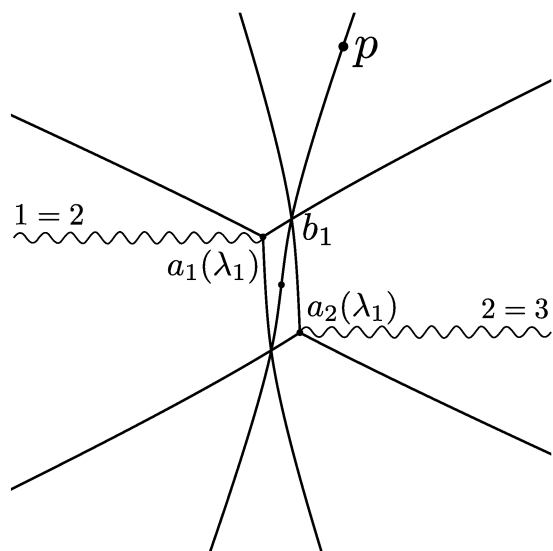
Figure 9. The Stokes geometry for the \text{BNR}_{\lambda_1} equation. (A wiggly line designates a cut to define \xi_i(x_1, \lambda_1) . For example, on a cut with the symbol “ 1 = 2 ” the numbering of \xi_1 and \xi_2 should be interchanged.)
