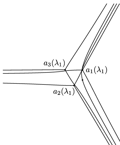
Figure 24. The ordinary Stokes curves and the third new Stokes curve of the \text{AKT}_{\lambda_1} equation shown in Figure 13.
