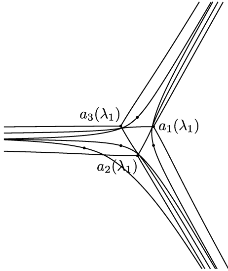
Figure 27. The Stokes geometry in question of the \text{AKT}_{\lambda_1} equation.
