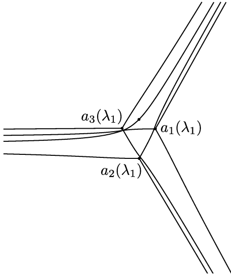
Figure 18. The Stokes geometry in question of the \text{AKT}_{\lambda_1} equation.
