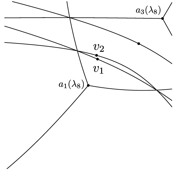
Figure 46. The enlarged version of Figure 45 around the turning point x_1 = a_1(\lambda_8) .
