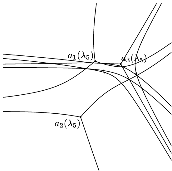
Figure 31. The Stokes geometry in question of the \text{AKT}_{\lambda_5} equation.
