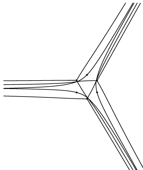
Figure 13. The Stokes geometry shown in Figure 12 with the new Stokes curves relevant to Stokes phenomena being added; the dot on a new Stokes curve designates the virtual turning point from which it emanates.
