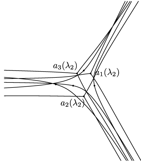
Figure 28. The Stokes geometry in question of the \text{AKT}_{\lambda_2} equation.
