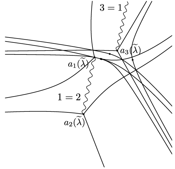
Figure 37. The Stokes geometry for the \text{AKT}_{\tilde{\lambda}} equation.
