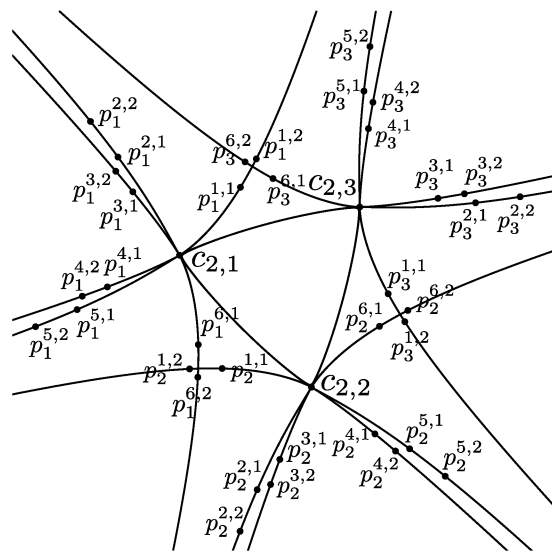
Figure 54. The labeling of zeros of (3.54).
