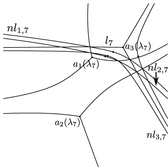
Figure 33. The Stokes geometry in question of the \text{AKT}_{\lambda_7} equation.
