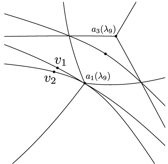
Figure 48. The enlarged version of Figure 47 around the turning point x_1 = a_1(\lambda_9) .
