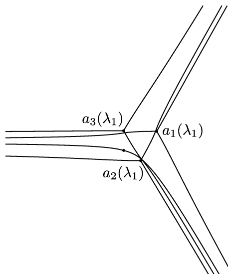
Figure 22. The ordinary Stokes curves and the second new Stokes curve of the \text{AKT}_{\lambda_1} equation shown in Figure 13.
