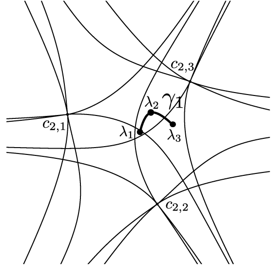
Figure 17. The path \gamma_1 and points \lambda_j ( j = 1, 2, 3 ) on it.
