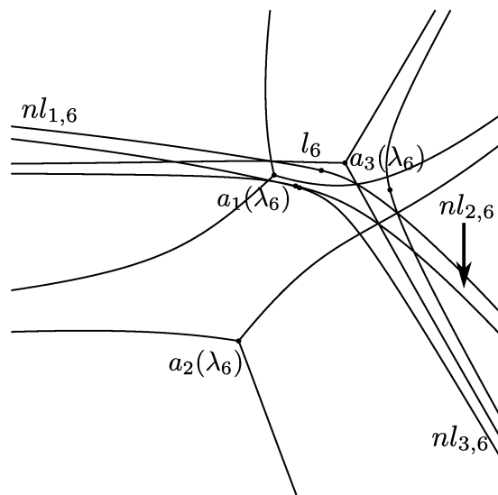
Figure 32. The Stokes geometry in question of the \text{AKT}_{\lambda_6} equation.
