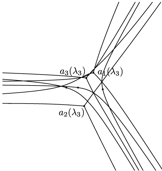
Figure 29. The Stokes geometry in question of the \text{AKT}_{\lambda_3} equation.
