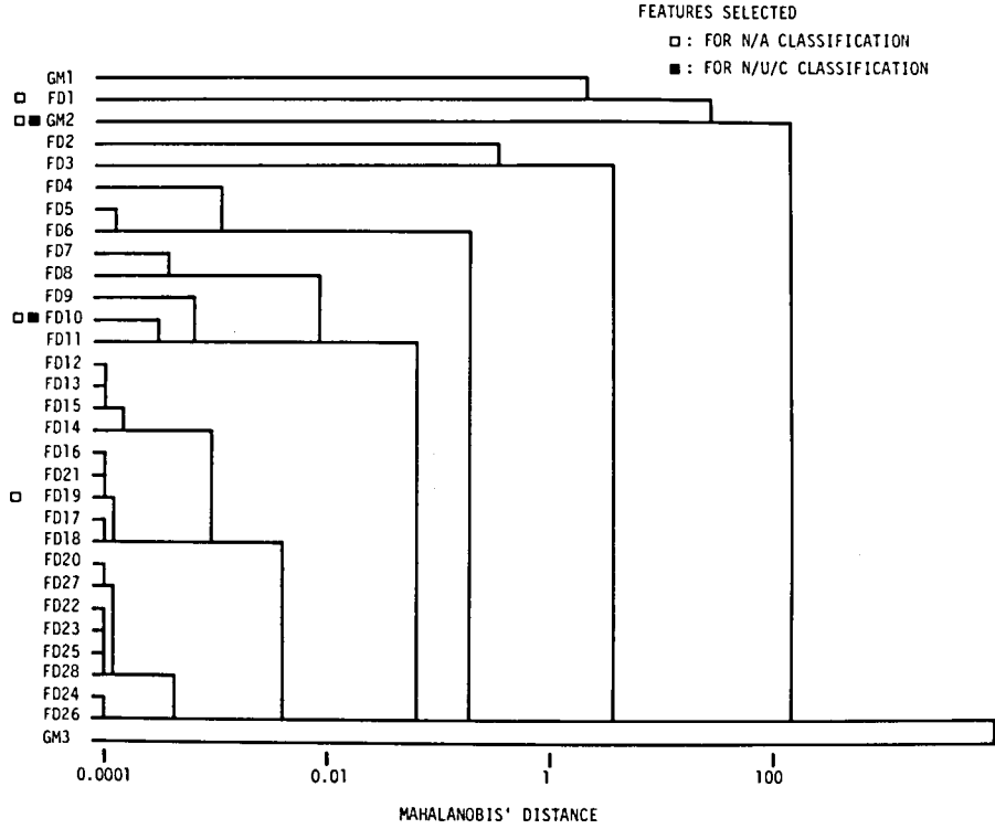
Fig. 4.7 A dendrogram of the clustering of the contour features.
