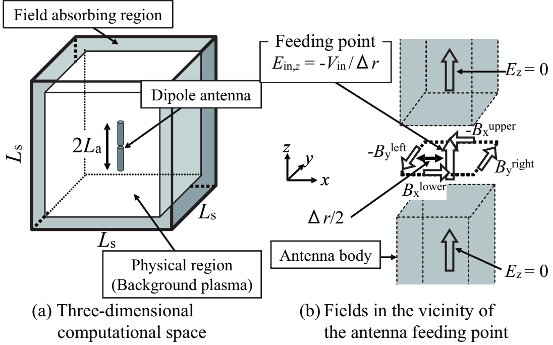
Figure 3.1: Model of the numerical simulation. (a) The dipole antenna is placed at the center of the simulation box. (b) The electric field E_{in,z} = -V_{in} / \Delta r is provided at the gap between two antenna elements.
