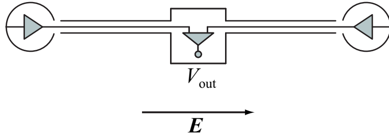
Figure 1.2: Schematic illustrations of a cylindrical wire antenna and a spherical double probe.
