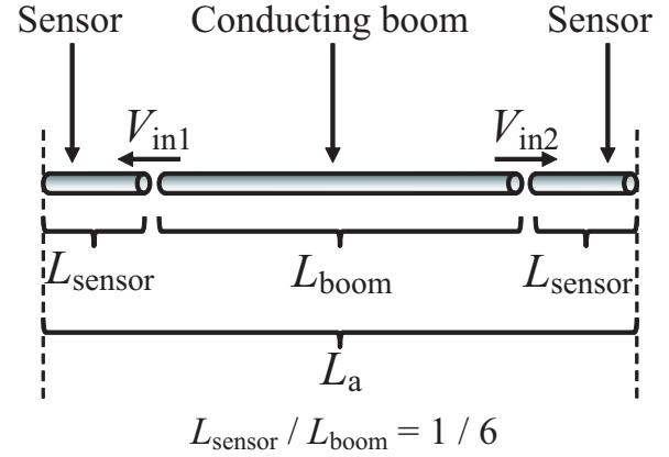
Figure 5.3: Wire antenna models examined in the computer experiments of the plasma wave reception. (a) Simple dipole antenna. (b) Linear-probe antenna.
