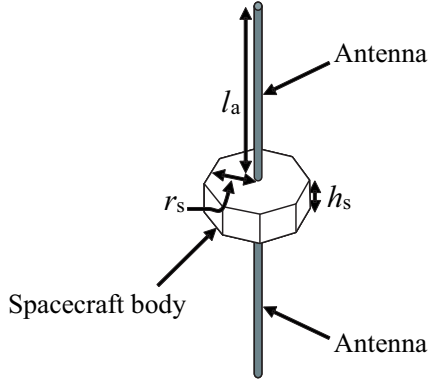
(a) Model of the antennas and the spacecraft (Perfect conductors)
