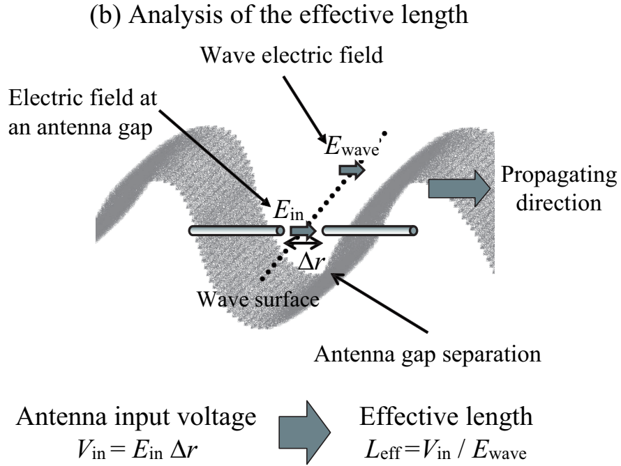
Figure 5.2: Model of computer experiments of the receiving antenna analysis. (a) Orientation of the antenna and the wavenumber vector. (b) Schematic illustration showing a calculation method of the effective length.
