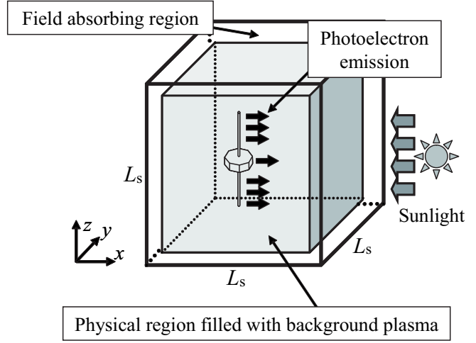
Figure 4.1: Three-dimensional simulation model for the antenna analysis in a photoelectron environment.
