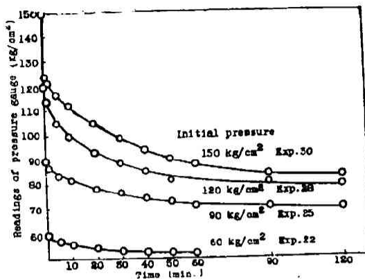
Fig. 5 Pressure change curves. P_{\text{NH}_3} : P_{\text{CO}_2} = 2 : 1, 170^\circ\text{C} .
