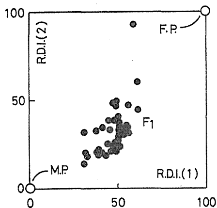
Fig. 4. Relationship between R. D. I. (1) [(Medial position of main resin duct/2 + Medial position of sub resin duct/total sub resin duct) / 2 × 100] and R. D. I. (2) [(Total medial position of resin duct/total resin duct) × 100]. Symbols are same as shown in Table 1.
