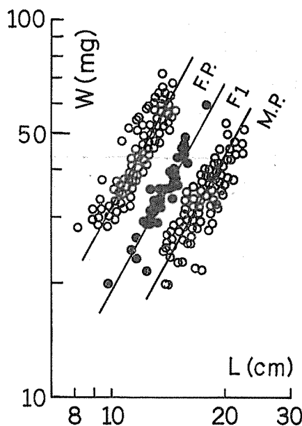
Fig. 3. Allometric correlations between length (L) and dry weight (W) of a needle. Symbols are same as shown in Table 1.
