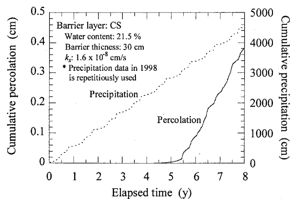
Fig. 5.14 Quantity of percolated water from the cover system with a CS barrier (water content of 21.5%, thickness of 30 cm) located in Owase
