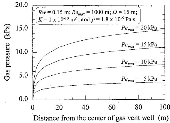
Fig. 7.10 Pressure profile beside a passive gas vent well with 30 cm in diameter
