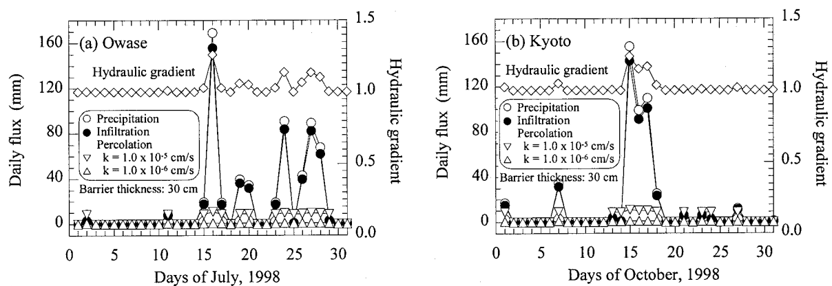
Fig. 4.10 Daily changes in the water balance in the daily cover systems with sludge barriers in (a) Owase and (b) Kyoto
