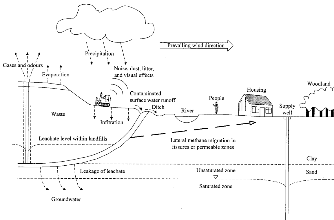
Fig. 2.9 General issues associated with landfills
