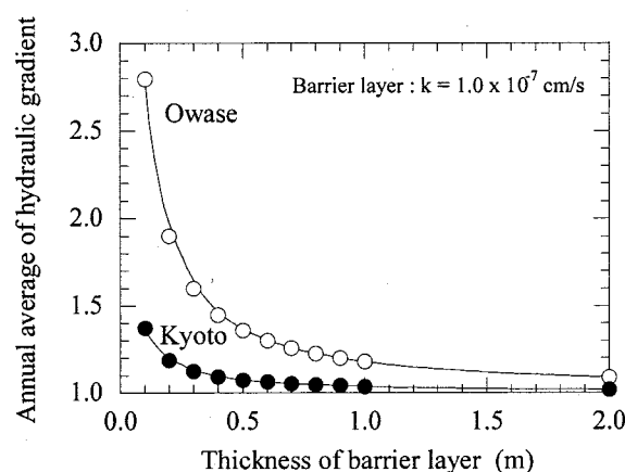
Fig. 4.6 Annual average hydraulic gradient for the thickness of sludge barriers in Owase and Kyoto
