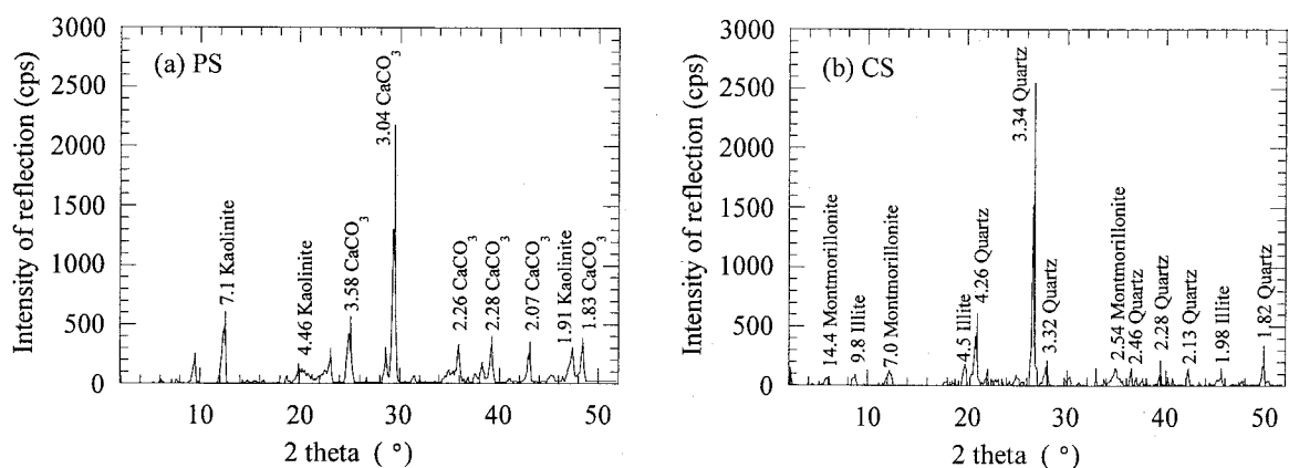
Fig. 3.13 X-ray diffraction patterns of (a) PS and (b) CS
