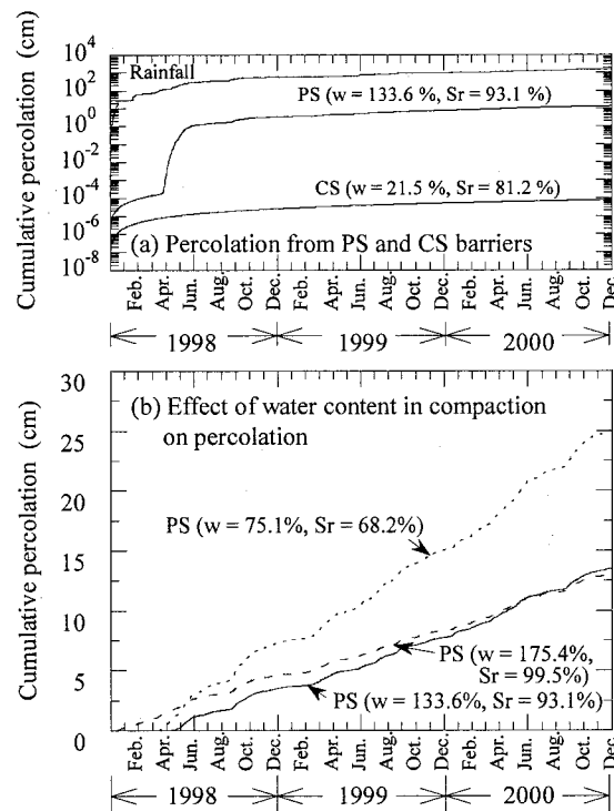
Fig. 5.12 Effects of sludge type and molding water content of the PS barrier on the quantity of percolation water
