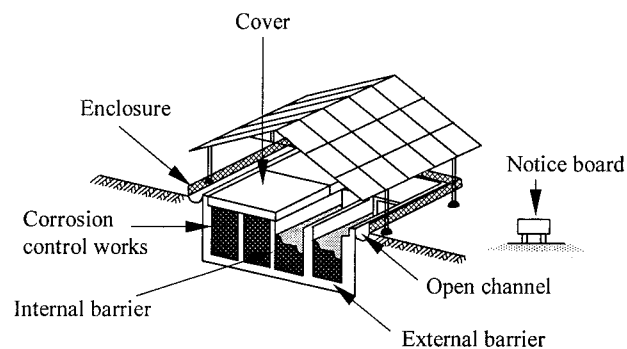
Fig. 2.8 Types of waste containment facilities in Japan
