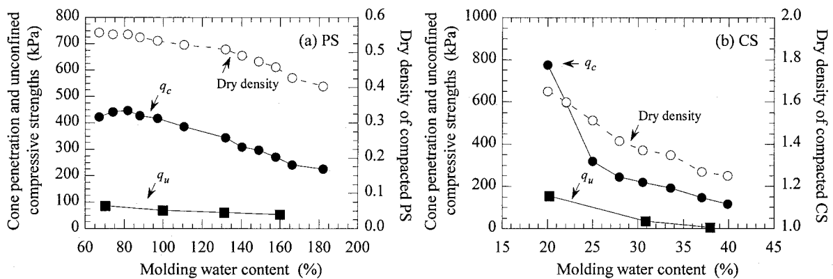
Fig. 3.5 Cone penetration strength, unconfined compressive strengths, and dry density of (a) PS and (b) CS compacted at different levels of molding water content
