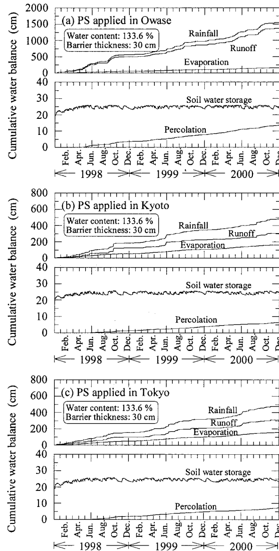
Fig. 5.11 Influence of weather conditions at each site on the results of the water balance analysis for cover systems with a PS barrier (water content of 133.6%, thickness of 30 cm)
