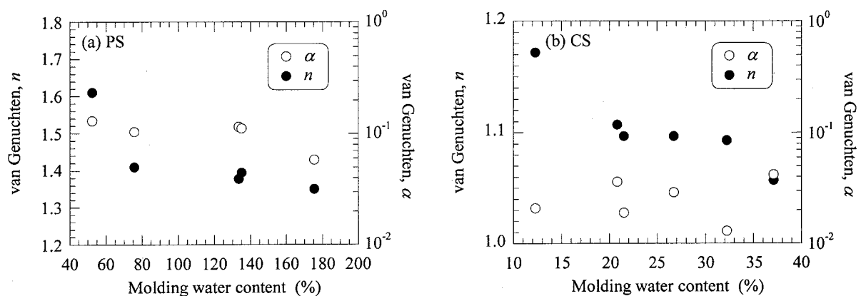
Fig. 5.6 Water content in compaction versus van Genuchten parameters for compacted (a) PS and (b) CS
