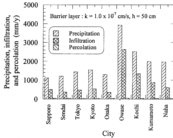
Fig. 4.4 Results of water balance analysis for final cover systems with a sludge barrier at each site
