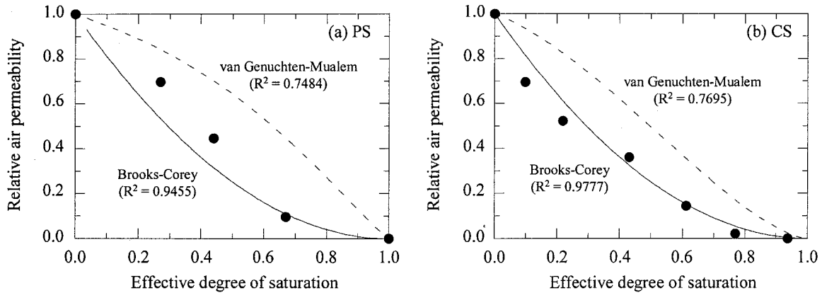
Fig. 7.6 Comparison of experimental data and fitted lines based on the Brooks-Corey and the van Genuchten-Mualem expressions for (a) PS and (b) CS
