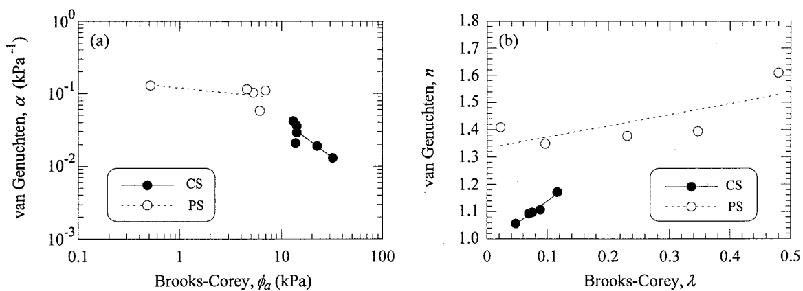
Fig. 5.5 Relationship between van Genuchten and Brooks-Corey parameters represented by (a) \alpha versus \phi_a and (b) n versus \lambda
