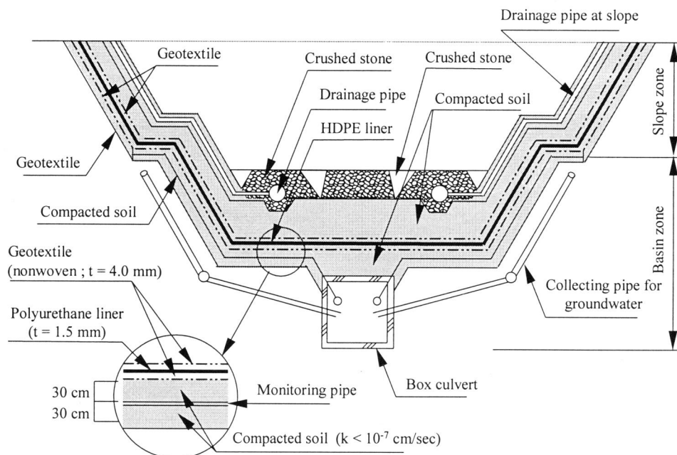
Fig. 2.11 Composite bottom liner system used in Hinode landfill site, Tokyo, Japan (adopted from Kamon, 1999)
