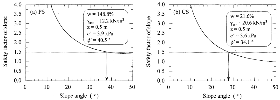
Fig. 3.7 Safety factor of slope composed of compacted (a) PS or (b) CS as barrier layer material
