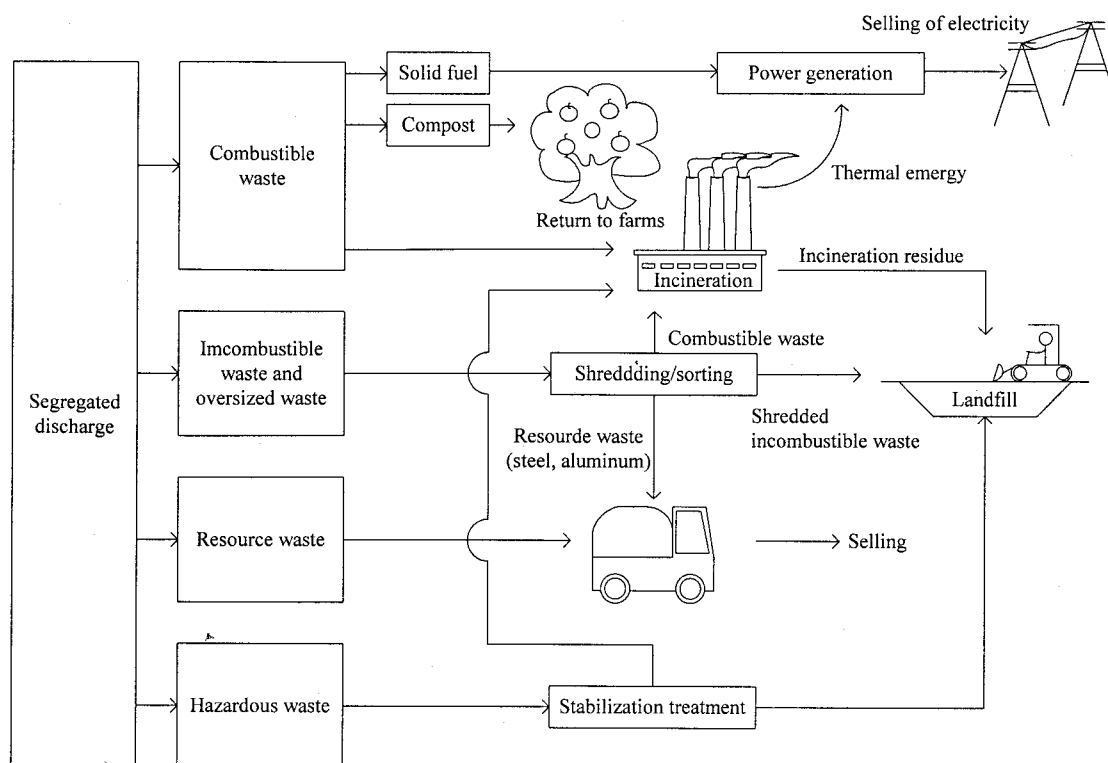
Fig. 2.2 Treatment and disposal flow of municipal solid waste (MSW)
