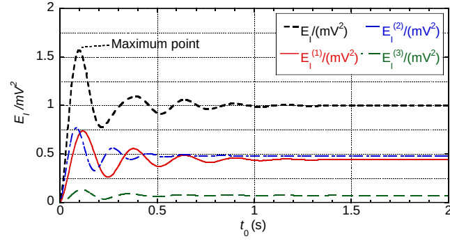
Fig.10 Input energies to overall system, main structure, substructure and connecting damper with respect to interval of double impulses
