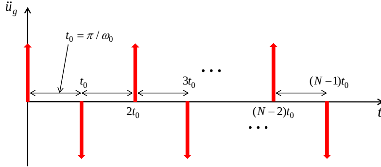
Fig.12 N impulses as simplification of long-duration ground acceleration
