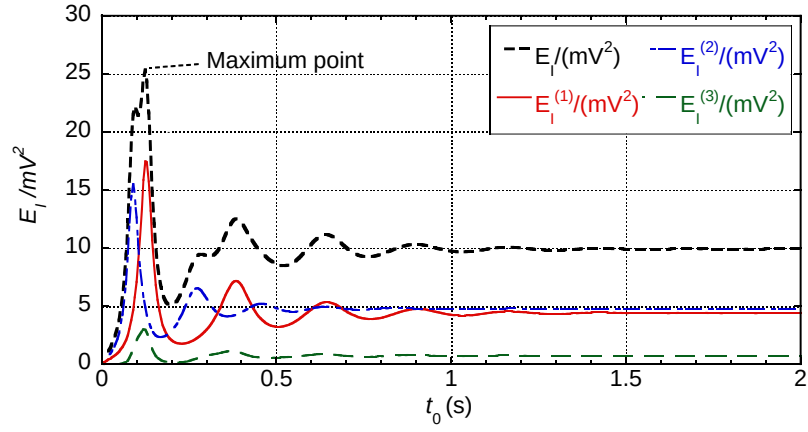
Fig.15 Input energies to overall system, main structure, substructure and connecting damper with respect to interval of 20 impulses
