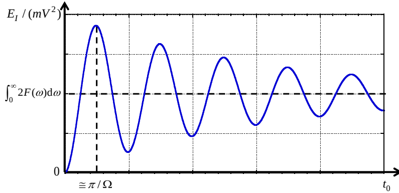
Fig.8 Schematic diagram of normalized earthquake input energy with respect to interval of double impulse
