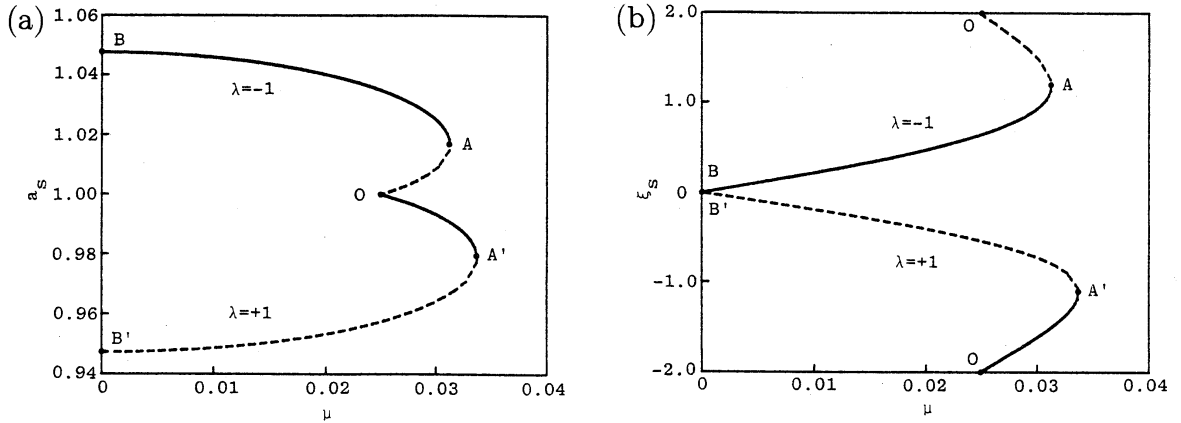
FIG.7. Plot of the stationary amplitude a_s and the stationary position \xi_s as a function of \mu for the values of the parameters \Gamma = 1.0 and \gamma = 0.05 .
