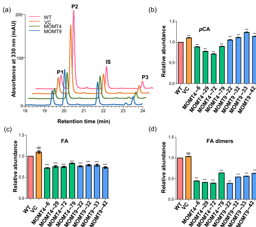
Figure 4 Wall-bound hydroxycinnamates released by mild acidolysis. (a) A portion of UV-LC-MS profile of phenolic extracts recovered after trifluoroacetic acid (TFA)-mediated mild acidolysis and saponification of cell wall residues from 1.5-month-old WT, VC, MOMT4 and MOMT9 overexpression plants. P1, p -coumarate (pCA); P2, ferulate (FA); P3, ferulate dehydromer. IS, internal standard. (b–d) Relative abundance of the phenolics pCA (b), FA (c) and FA dimers (d) released from the arabinoxylan-bound in MOMT4 and MOMT9 overexpression lines, compared to the WT. Quantifications of pCA and FA were based on their UV absorptive peak area, while quantification of FA dimers was based on the extracted ion abundance at m/z 385.09. The average amount detected in the WT was set as 1. Data are represented as mean \pm s.e. from two biological replicates with three technical repeats for WT and VC plants and three technical repeats for individual MOMT4 and MOMT9 overexpression lines. *** indicates statistically significant difference with P < 0.001 , compared to the WT (one-way ANOVA test; Tukey's multiple comparison test). NS, not significant.
